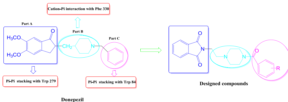
Figure 3. Design of compounds 4a-4j according to the pharmacophoric necessities of donepezil
