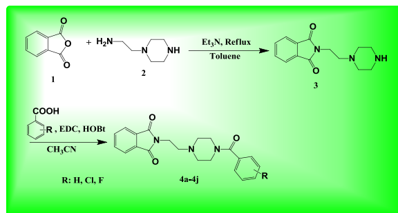
Scheme 1. Synthetic pathway for preparation of 4a-4j
