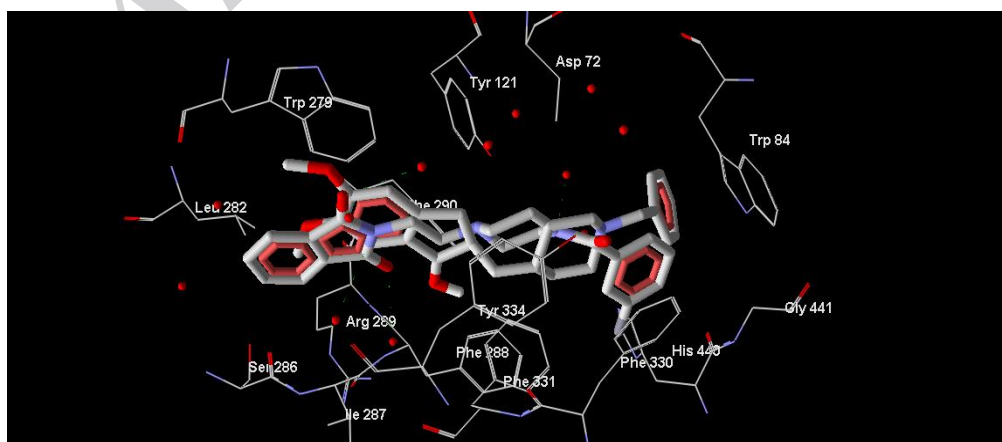
Figure 5. Superimposition of compound 4e with structure of donepezil in the active site of AChE
