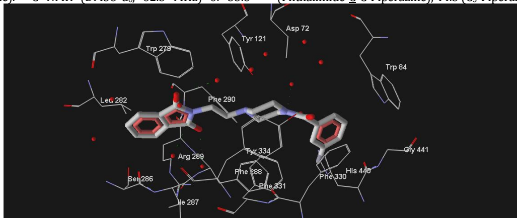
Figure 4. Structure of compound 4e (3-fluoro derivative) in the active site of acetylcholinesterase. The ligand is rendered as stick and the amino acids of the active site of AChE is presented as wireframe. Water molecules provided as red core
