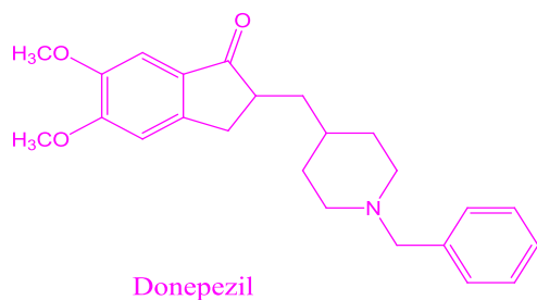
Figure 1. Structures of acetylcholinesterase inhibitors in the market
