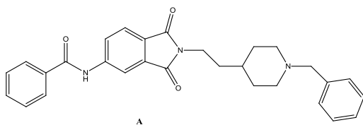
Figure 2. Structure of a phthalimide based compound as acetylcholinesterase inhibitor
