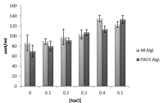
Figure 1. The alginate lyase activity from isolates PAO1 and 48 at different NaCl concentrations
