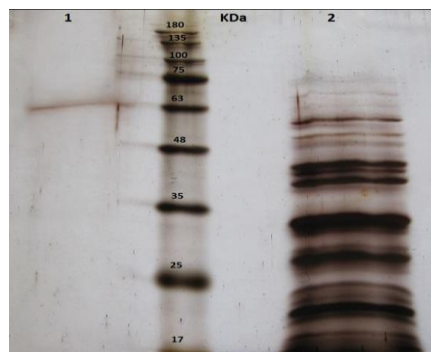
Figure 7. SDS-polyacrylamide gel electrophoresis of alginate lyase. Line 1: The purified enzyme by affinity chromatography; line 2: The crude extract
