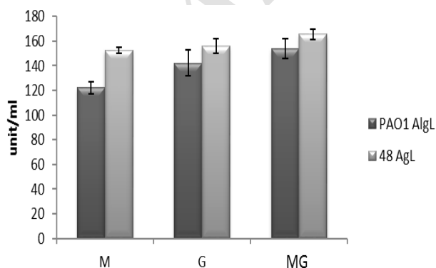
Figure 4. The alginate lyase assay of strain 48 and strain PAO1 using polyM, polyG and poly MG blocks of sodium alginate as substrates
