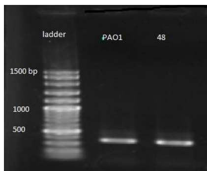
Figure 6. PCR analysis of poly M conserved region in strain PAO1 and strain 48
