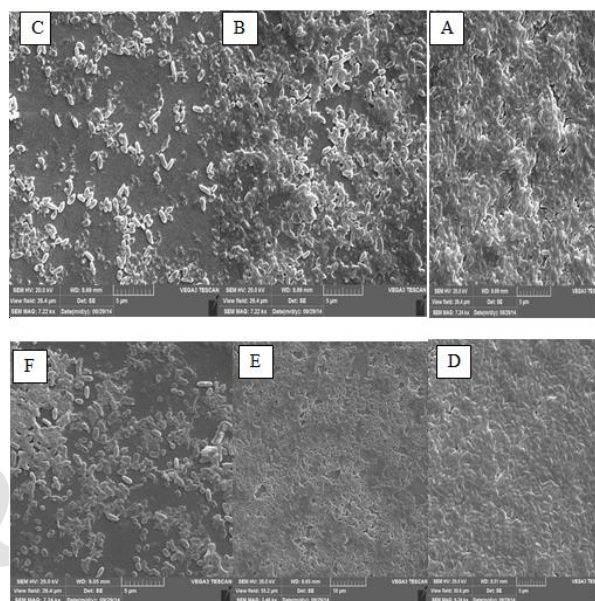
Figure 9. Representative SEM images of A) 24- hr biofilm from Pseudomonas aeruginosa PAO1, B) The removal of 24- hr PAO1 biofilm by the enzyme extract of strain 48, C) The prevention of PAO1 biofilm formation by the enzyme extract of strain 48, D) 24- hr P. aeruginosa 48 biofilm, E) The removal of 24- hr strain 48 biofilm by the enzyme extract of strain 48, F) The prevention of strain 48 biofilm formation by the enzyme extract of strain 48
