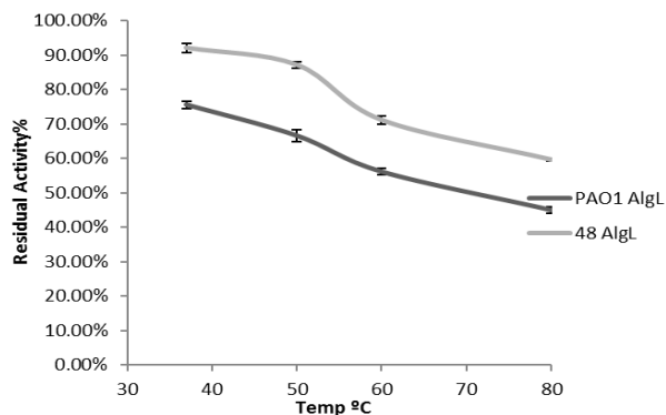
Figure 2. The residual activity of the alginate lyase from isolates PAO1 and 48 after 1 hr incubation at different temperatures
