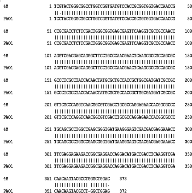
Figure 5. The alignment between the alginate lyase sequences of strain 48 with conserved sequence of PAO1 strain
