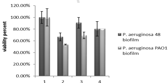
Figure 8. The influence of the enzyme extracts from strain 48 on Pseudomonas aeruginosa 48 and Pseudomonas aeruginosa PAO1 biofilm. 1) 24- hr biofilm 2) The elimination of 24- hr biofilm by enzyme extract from strain 48 3) The inhibition of biofilm formation by the enzyme extract from strain 48 4) The removal of 24- hrs biofilm by the purified enzyme (0.043 mg/ml)
