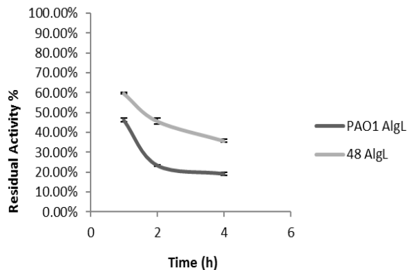
Figure 3. The residual activity of the alginate lyase from isolates PAO1 and 48 at 80 °C at various times
