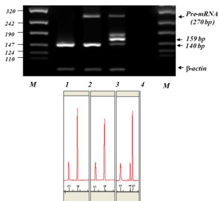
Figure 4. RT-PCR analysis of the EGFP assay constructs. Lane 1, 2 and 3 correspond to RT-PCR analysis on pEGFP C1, pEGFP C1+ I wt and pEGFP C1+ I 1-110 , respectively. Lane M corresponds to molecular marker VIII (Roche). Lower panel illustrates the capillary electrophoresis of the corresponding lanes
