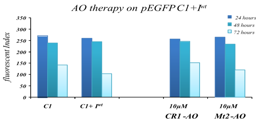
Figure 7. Time dependent effect of antisense oligonucleotide (AO) treatment on fluorescent index (FI) in pEGFP C1 + I wt transfected cells. EGFP activity in K562 cells co-transiently transfected with AOs and pEGFP + I wt plasmid. The activity of EGFP was normalized to total cellular EGFP fluorescence and is presented as FI. This figure shows that CR1-AO and Mt2-AO did not influence EGFP expression in cells co-transfected with pEGFP C1 + I wt plasmid
