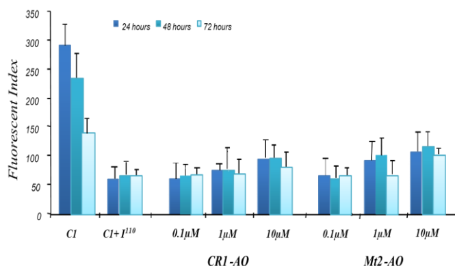
Figure 6. Time and dose-dependent effect of antisense oligonucleotide (AO) treatment on fluorescent index (FI) with pEGFP C1 + I I-110 transfected cells. EGFP activity in K562 cells co-transfected with AOs and pEGFP C1 + I IVSI-110 plasmid (n=2). The activity of EGFP was normalized to total cellular EGFP fluorescence and is presented as FI
