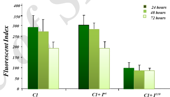
Figure 3. Comparison of FI values following transient transfection of EGFP plasmids. pEGFP C1, pEGFP C1+ I wt and pEGFP C1+ I 1-110 in K562 cells. Multiplying the percentage of EGFP positive cells with median peak fluorescence was used to derive FI. The FI values following transfection were calculated at 24 hrs, 48 hrs and 72 hr (Results represent the average of three independent experiments \pm SD)
