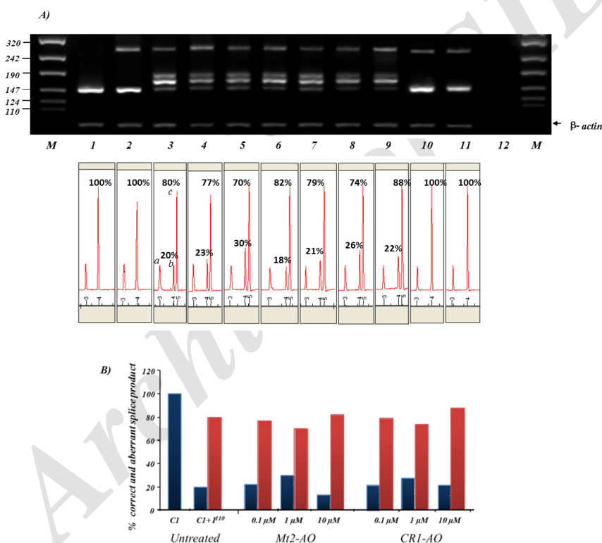
Figure 8. Dose-dependent effects of antisense oligonucleotide (AO) treatment on pEGFP C1 + I 1-110 transfected cells. (A) RT-PCR analysis on K562 cells co-transiently transfected with AOs and pEGFP C1 + I IVSI-110 plasmid. Lane 1-3 correspond to untreated and pEGFP C1 and pEGFP C1 + I wt , pEGFP C1 + I IVSI-110 , respectively. Lanes 4-5 correspond to cells co-transfected with pEGFP C1 + I IVSI-110 and Mt2-AOs at 0.1, 1 and 10 μM, respectively. Lanes 6-9 correspond to cells pEGFP C1 + I IVSI-110 co-transfected with CR1-AOs at 0.1, 1 and 10 μM, respectively. Lane 10 and 11 correspond to pEGFP C1 + I wt co-transfected with Mt2-AO and CR1-AO at 10 μM concentration, respectively. (B) Relative amounts between normal (blue) and aberrant (red) splice RT-PCR products following AO therapy. Using Mt2-AO and CR2-AO at 1 μM resulted in 10% and 6% increase in normal splicing, respectively
