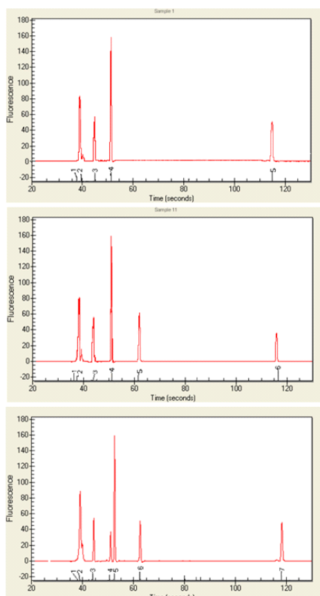
Figure 5. Analysis of RT-PCR products by capillary electrophoresis following transient transfection of EGFP plasmids into K562 cells. A) pEGFP C1. B) pEGFP C1 + I wt , C) pEGFP C1 + I I-110 . Peaks "a" and "f" correspond to lower (15 bp) and upper (1500 bp) internal markers in capillary electrophoresis. Peak "b" corresponds to \beta -actin. Peak "c" corresponds to the correctly spliced product (140 bp). Peak "d" in panel C corresponds to the aberrantly spliced product (159 bp). Percentages (19.6% and 80.4%) in panel C correspond to correctly and aberrantly product, respectively. Peak "e" in panel B and C indicate to pre mRNA in pEGFP C1 + I wt and pEGFP C1 + I I-110 (270 bp)
