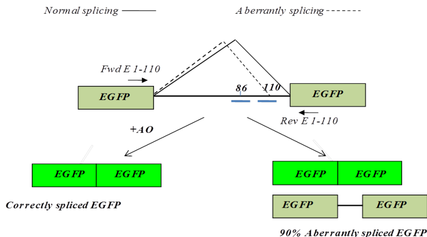
Figure 1. Splicing of EGFP-IVSI-110 mRNA. Schematic diagram illustrating EGFP pre-mRNA containing intron I of \beta -globin carrying the G>A splicing mutation at nucleotide 110. The mutation activates an aberrant splice site. Short bars at position 86 and 110 of intron I represent targeted 2'-O-Me phosphorothioate antisense oligonucleotides (AOs), which have been targeted to redirect aberrant splicing. Primers Fwd E 1-110 and Rev E 1-110 were used in RT-PCR
