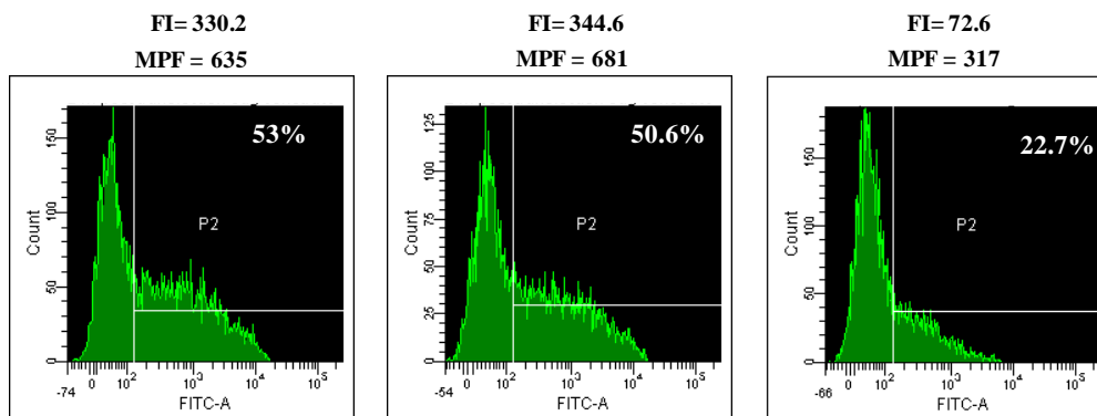
Figure 2. Representative flowcytometric analysis of EGFP expression in splicing assays system. Panel A corresponds to K562 cells transfected with pEGFP C1, panel B corresponds to K562 cells transfected with pEGFP C1+ I wt and panel C corresponds to K562 cells transfected with pEGFP C1+ I 1-110
