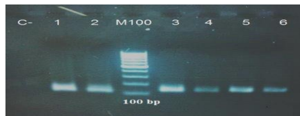
Figure 4. Representative ethidium bromide-stained gel electrophoresis confirmed the size of all generated PCR products was at 134 bp for \beta -actin in 1 and 2 columns, 130 bp for GAD65 in 3 and 4 columns and 113 bp for GAD67 in 5 and 6 columns. Lane C- is negative control and lane M100 is 100-bp DNA marker
