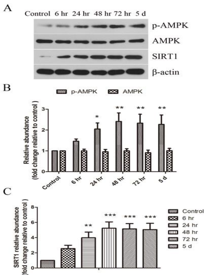
Figure 4. Effect of mechanical injury on protein levels of phosphorylated-AMP-activated protein kinase and sirtuin 1 in primary spinal cord neurons. (A) The levels of p-AMPK and SIRT1 in primary spinal cord neurons were evaluated by Western blot assay. \beta -actin was used as a loading control. (B)&(C) The gray intensities of the bands were statistically analyzed and shown. The results shown represent at least three independent experiments. Each value represents the mean \pm SD (n=3). * P <0.05, ** P <0.01, *** P < 0.001, versus the control group
