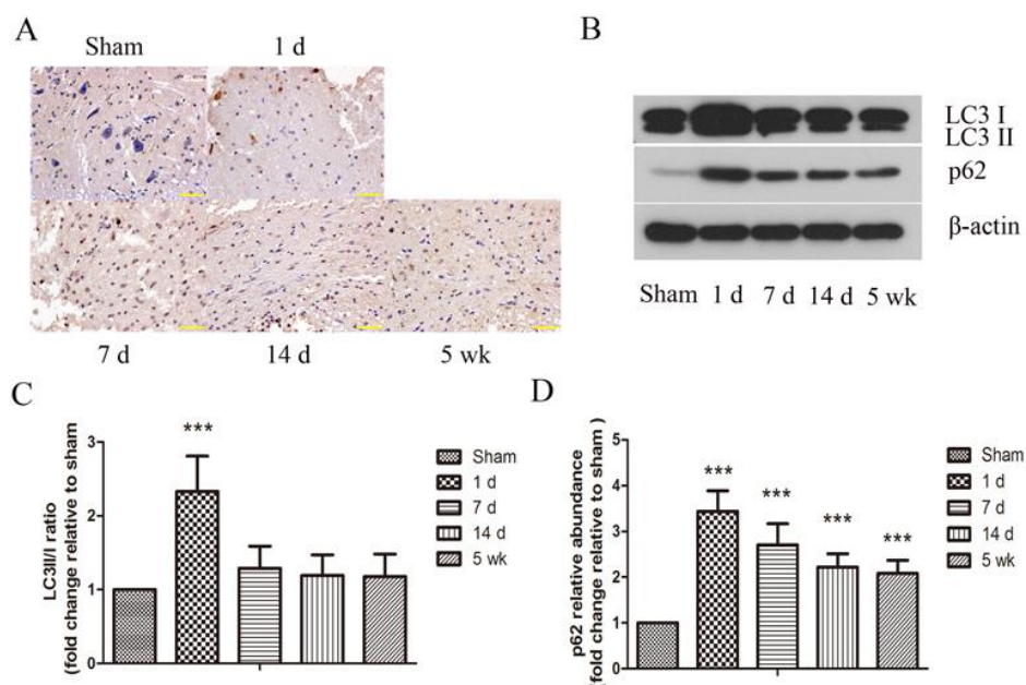
Figure 1. The changes in apoptosis and autophagy flux in spinal cord tissue after spinal cord injury. (A) The apoptosis in spinal cord tissue was detected by TUNEL staining (magnification 400x). (B) The protein levels of LC3I, LC3II and p62 in spinal cord tissue were assessed by Western blot assay. \beta -actin was used as a loading control. (C)&(D) The gray intensities of the bands were statistically analyzed and shown scale bar in A is 50 \mu m. The results shown represent at least three independent experiments. Each value represents the mean \pm SD (n=6) *** P <0.001, versus the sham group
