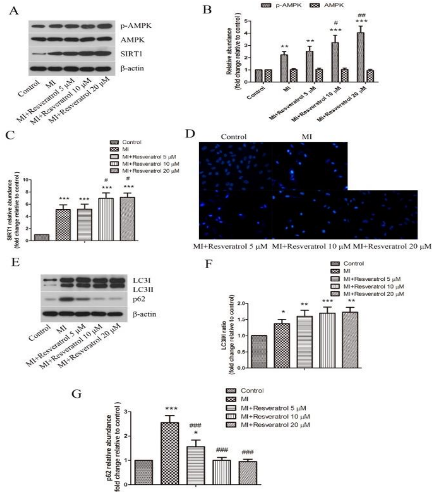
Figure 5. Activation of AMP-activated protein kinase/sirtuin 1 pathway by resveratrol alleviated mechanical injury-induced cell damage and impaired autophagy flux in primary spinal cord neurons. (A-C) The protein levels of p-AMPK and SIRT1 in primary spinal cord neurons were assessed by Western blot assay and the statistical analysis of the gray intensities of the bands were shown. \beta -actin was used as a loading control. (D) The nucleus damage induced by MI in primary neurons of spinal cord was observed by Hoechst 33342 staining. (E-G) The protein levels of LC3I, LC3II and p62 in primary spinal cord neurons were assessed by Western blot assay. \beta -actin was used as a loading control. The gray intensities of the bands were statistically analyzed and shown. The results shown represent at least three independent experiments. Each value represents the mean \pm SD (n= 3). * P <0.05, ** P <0.01, *** P <0.001, versus the control group. # P <0.05, ## P <0.01, ### P <0.001, versus the MI group
