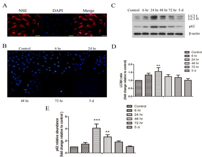
Figure 3. The cell damage and impaired autophagy flux induced by mechanical injury in primary spinal cord neurons. (A) The primary spinal cord neurons were identified by immunofluorescence staining of NSE (magnification 400x). (B) The nucleus damage induced by MI in primary neurons of spinal cord was observed by Hoechst 33342 staining. (C-E) The protein expressions of LC3I, LC3II and p62 in primary spinal cord neurons were determined by Western blot analysis. \beta -actin was used as a loading control. The gray intensities of the bands were statistically analyzed and shown. Scale bar in A is 50 \mu m. The results shown represent at least three independent experiments. Each value represents the mean \pm SD (n=3). ** P <0.01, *** P <0.001, versus the control group
