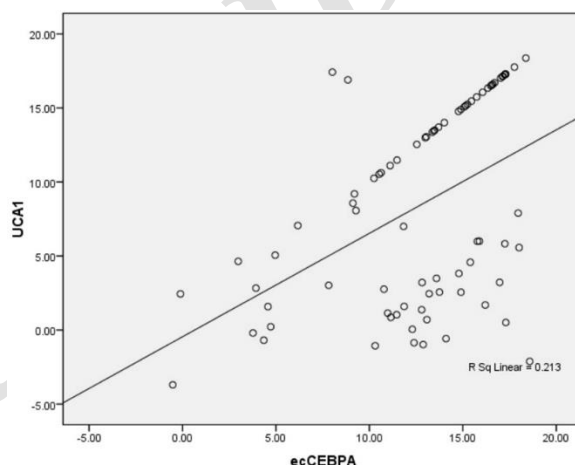
Figure 4. Correlation analysis of lncRNAs UCA1 and ecCEBPA gene expression levels ( P -value=0.000, r=0.46 )
