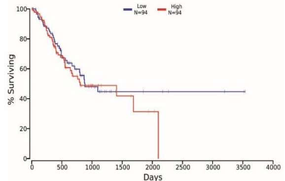
Gastric cancer ( p value= 9.90e-01 )
