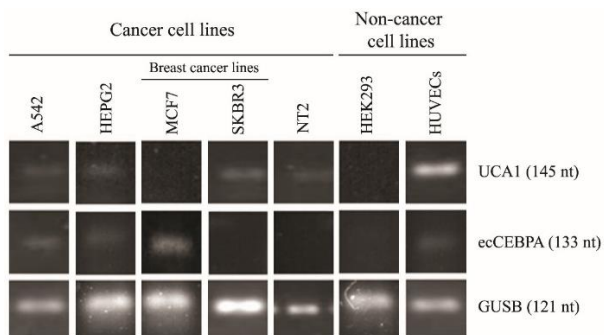
Figure 1. Expression of ecCEBPA , UCA1 , and GUSB transcripts in various cell lines. Electrophoresis results of ecCEBPA , UCA1 , and GUSB PCR products on the agarose gel are presented in the figure
