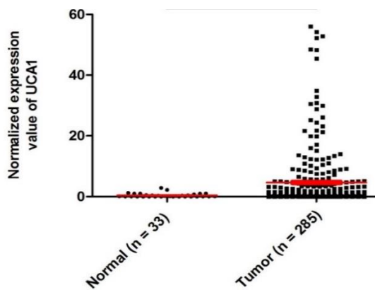
Figure 5. Relative expression of UCA1 in tumoral and non-tumoral gastric tissue samples in the TCGA database. UCA1 was found to be highly overexpressed in tumoral tissues compared with normal tissues in the TCGA RNA-seq data ( P < 0.0001 )
