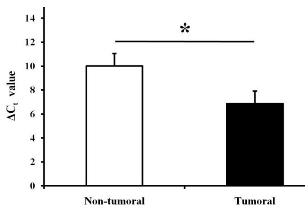
Figure 2. Relative expression of UCA1 in tumoral and non-tumoral gastric tissue samples (n=40). A lower \Delta C_t value shows higher expression levels. Values shown represent the mean \pm SEM. Asterisk represents a statistically significant difference ( P \leq 0.05 ) Error bars stand for standard error of mean (SEM)
