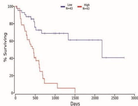
Pancreatic Adenocarcinoma ( p value= 4.50e-06 )
