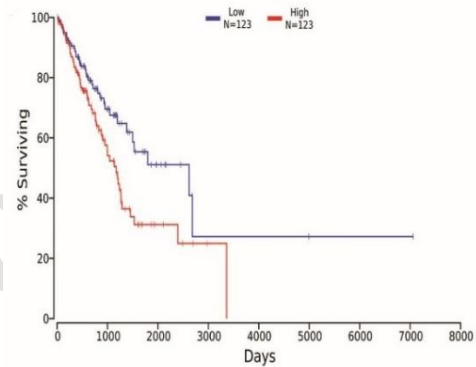
Lung Adenocarcinoma ( p value= 7.30e-03 )
