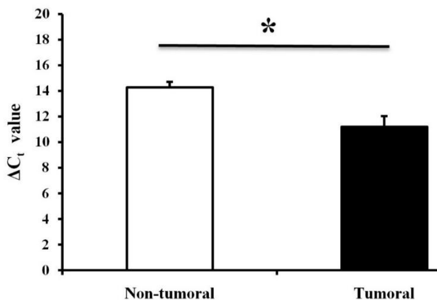
Figure 3. Relative expression of ecCEBPA in tumoral and non-tumoral gastric tissue samples (n=40). A lower \Delta C_t value shows higher expression levels. Values shown represent the mean \pm SEM. Asterisk represents a statistically significant difference ( P \leq 0.05 ) Error bars stand for standard error of mean (SEM)
