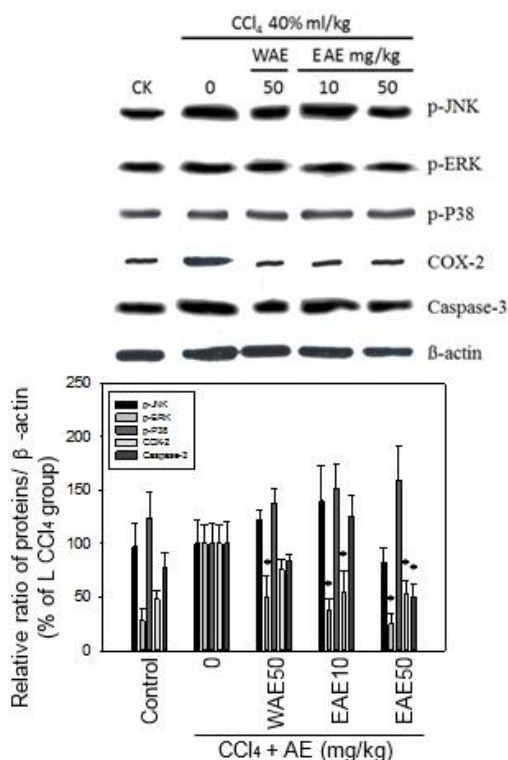
Figure 6. AC extract inhibited CCl 4 -induced phospho-ERK MAP kinase, COX-2 and caspase-3 under CCl 4 stress. EAE and WEA both extracts reduced the p-ERK activation, and EAE inhibit COX-2, and caspase-3 levels better than WEA in the liver samples. Data are expressed as mean ± SEM of three independent experiments. *:P<0.05 as compared to CCl 4 control
