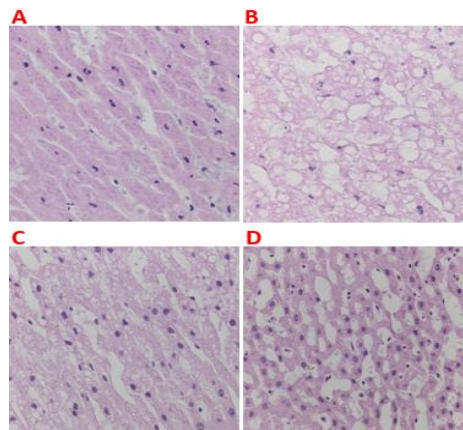
Figure 5. Protective effect of the Antrodia cinnamomea (AC) extract on CCl 4 -induced hepatic injury. Histopathology of liver slices from rats from (A) no treatment control group; (B) the CCl 4 group, (C) the EAE group, and (D) the WAE group. The photographs show the liver section with 200× magnification
