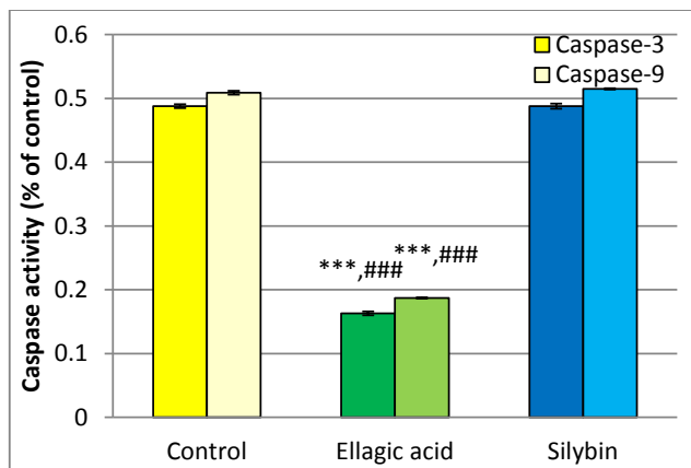
Figure 3. Effect of EA and silybin on caspase-3 and -9 activities on islet of Langerhans cells.***significant difference from the control group at P<0.001 .###significant difference from silybin group at P<0.001
