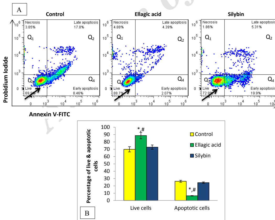
Figure 2. Flow cytometry assessment of effects of EA and silybin on pancreatic cells. (A) Changes in percent of live, apoptotic and necrotic populations of the islets cells are exhibited. Left down square shows live cells with FITC - and PI - , right down square indicates early apoptotic cells with FITC + and PI - , above right square displays late apoptotic cells with FITC + and PI + and above left square expresses necrotic cells with FITC - and PI + . (B) Percentage of live and apoptotic cells. *significant difference from control group at P < 0.05 . #significant difference from silybin group at P < 0.05
