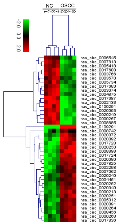
Figure 1. CircRNAs expression profile in oral squamous cell carcinoma tumor tissues. OSCC-related circRNAs were selected out based on FDR \leq 0.001 and fold change \geq 2 or fold change \leq 0.5 . 41 circRNAs were differentially expressed between OSCC tissues and normal tissues. The heat map showed the 41 differentially expressed circRNAs, red indicating high expression and green indicating low expression
