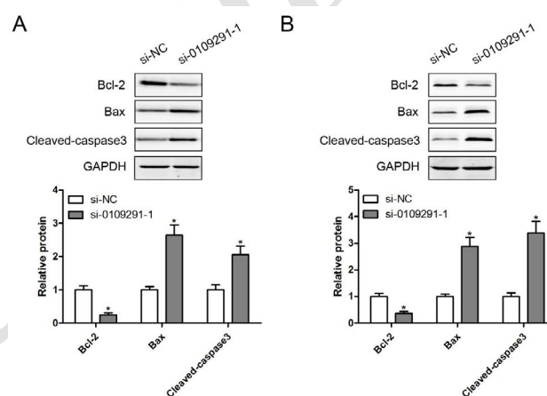
Figure 6. Inhibition of hsa_circ_0109291 regulated apoptosis-related protein expression. After transfection with si-0109291-1 and si-NC, protein expression of Bcl-2, Bax, and Cleaved-caspase3 was measured by Western blotting in SCC4 (A) and CAL27 (B) cells for 24 hr. * P < 0.05
