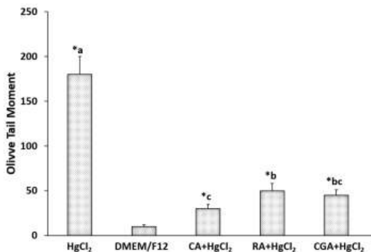
Figure 2. Olive tail moment of precision-cut kidney slices exposed to mercuric chloride and treated with phenolic acids. The olive tail moment was determined from each of the treatments. HgCl 2 (15 μM) was used as control of damage; negative control was DMEM/F12 medium. Kidney slices were co-incubated separately with 15 μM HgCl 2 and CA (3 μg/ml), RA (6 μg/ml) and CGA (9 μg/ml). Values represent the mean and standard deviation of 100 cells/ treatment. Normality of the data was evaluated with the Shapiro-Wilks test. The T Student's Test was applied, and significant differences were analyzed with the Tukey's test ( P \leq 0.01 ). A significant difference exists between slices treated with HgCl 2 (a) and those co-incubated with the PAs (b, c, d). CA exhibited the biggest difference (c)
