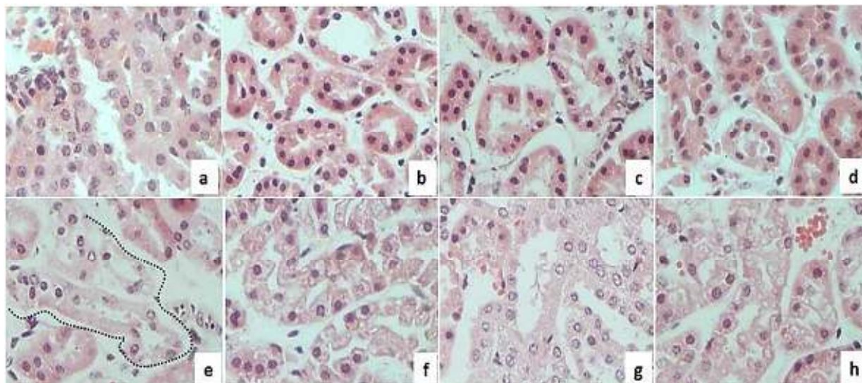
Figure 4. Histopathologic analysis of precision-cut kidney slices treated with mercuric chloride and phenolic acids. PCKS were incubated in the presence of (a) cell culture medium, (b) 9 µg/ml CGA, (c) 3 µg/ml CA, (d) 6 µg/ml RA, (e) 15 µM HgCl 2 , (f) CGA+HgCl 2 , (g) CA+HgCl 2 , and (h) RA+HgCl 2 . Untreated slices showed morphologic characteristics of normal tissue, as well as preserved tubular structure (a). Slices incubated in the presence of phenolic acids alone show no signs of damage or morphological alterations (b, c, d). In contrast, mercury induced interstitial edema, tubular necrosis and the presence of apoptotic nuclei (e), dotted lines. In slices co-incubated with HgCl 2 and compounds, the damage induced by mercury was ameliorated; this was evident because of the conserved histologic structure, showing only mild interstitial edema. With CGA and RA hydropic degeneration was observed, whereas, with CA, less degenerative changes were observed (f, g, h). H&E stain. Total magnification 400X
