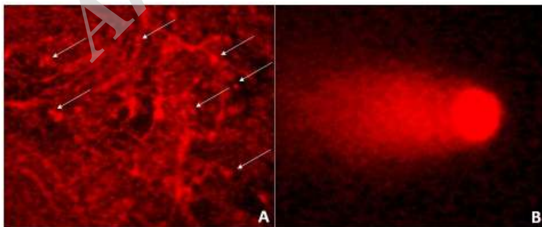
Figure 1. Fluorescent microscope images of tissue slices for the comet assay. PCKS were incubated with 15 \mu\text{M} HgCl 2 and processed for comet assay with the conventional technique (a), where a mass of tissue contains many renal cells trapped on the stroma (arrows) which are not appropriated for visual scoring after the squashing method. (b) Cells released from a treated slice after completion of the procedure using the homogenization method with the saccharose buffer. Ethidium bromide stain. Total magnification A (100X), B (400X)
