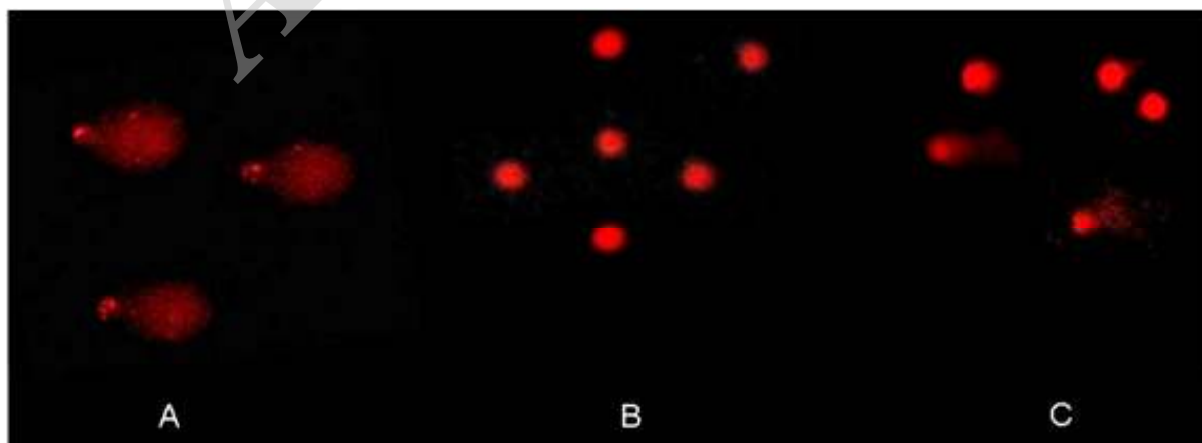
Figure 3. Comet assay from kidney slices incubated with mercuric chloride and phenolic acids. Representative cell images from PCKS incubated with 15 μM HgCl 2 showed the typical form of long-tail comets indicating DNA strand breaks in the cells (a). Untreated slices (b) showed round nuclei, with intact DNA, while in the kidney slices incubated with 3 μg/mL CA+15 μM HgCl 2 the damage was attenuated (c). Ethidium bromide stain. Total magnification (200X)
