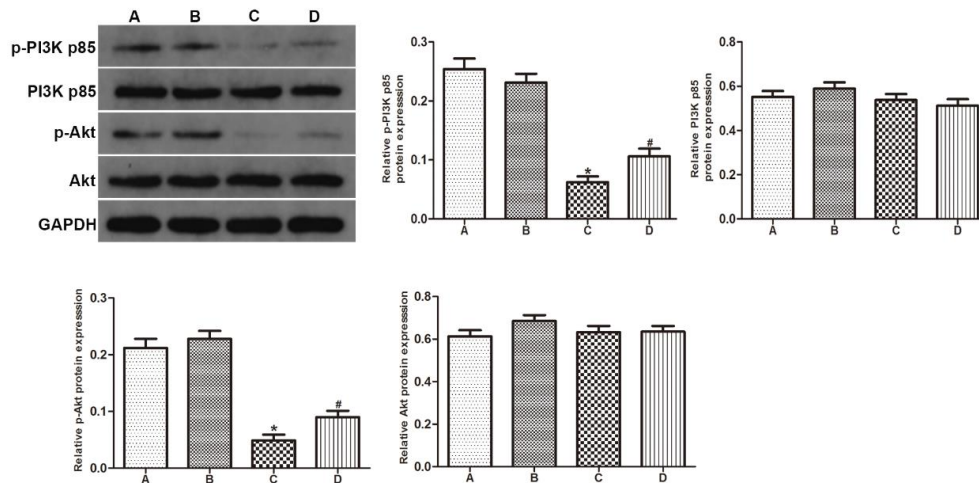
Figure 4. GYY4137 increased the phosphorylation of PI3K p85 and Akt. Protein expression levels of p-PI3K p85, p-Akt, PI3K p85 and Akt were studied by western blot analysis. (A) sham group, (B) sham+GYY4137 group, (C) VC group, (D) VC+GYY4137 group. * P < 0.05 vs group A; # P < 0.05 vs group C. VC, varicocele; GYY4137, Morpholin-4-ium 4 methoxyphenyl (morpholino) phosphonodithioate; PI3K, phosphatidylinositol 3-kinase; p-, phosphorylated
