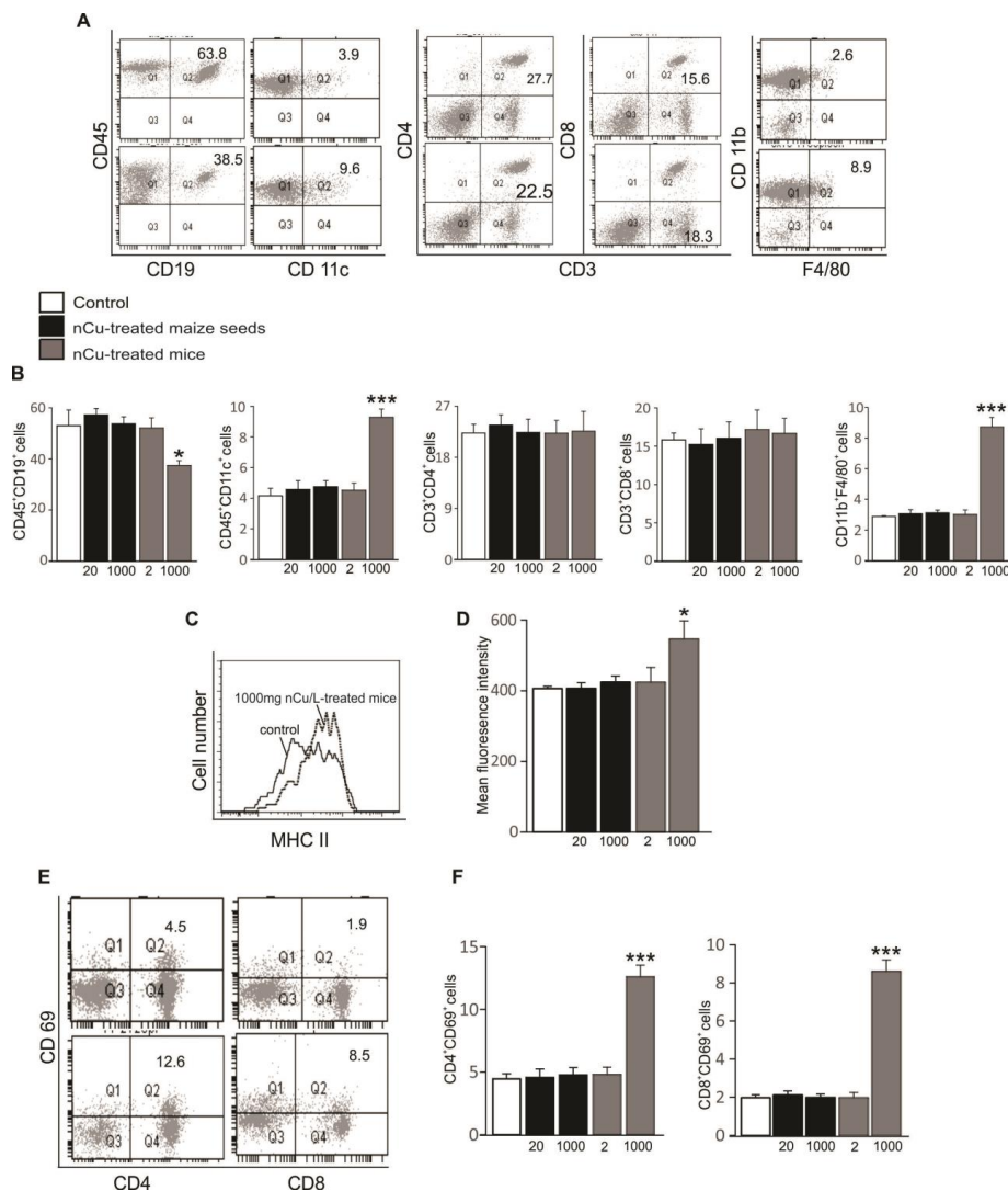
Figure 3. Effect of nano-copper on immune cell infiltration into mouse spleens. A. Original dot plots of CD45+CD19+, CD45+CD11c+, CD45+CD3+ CD4+, CD45+CD3+ CD8+ and CD45+CD11b+ F4/80+ cells recruited to spleens of mice, which were untreated (control, upper panels) and treated with 1000 mg/l nCu (lower panels). Numbers depict the percent of cells in the respective quadrants, acquired within the dead cell gate. B. Arithmetic means (n=4-5) of percentages of CD45+CD19+, CD45+CD11c+, CD45+CD3+ CD4+, CD45+CD3+ CD8+ and CD45+CD11b+ F4/80+ cells recruited to spleens of mice, which were left untreated (control, white bars) or fed with grain maize derived from 20 mg/kg dry weight (DW) or 1000 mg/kg DW nCu-treated seeds (black bars) or treated with nCu at dose of 2 mg/l or 1000 mg/l (grey bars). * (P<0.05) and *** (P<0.001) represent significant differences from control group, ANOVA. C. Histogram of major histocompatibility complex (MHC) class II expression was obtained by FACS analysis in a representative experiment on control (solid line) and 1000 mg nCu/l-treated splenic leukocytes (dotted line). D. Arithmetic means ± SEM (n=5) of mean fluorescence intensity (MFI) of splenic leukocytes in mice, which were left untreated (control, white bars) or fed with grain maize derived from 20 mg/kg DW or 1000 mg/kg DW nCu-treated seeds (black bars) or treated with nCu at dose of 2 mg/l or 1000 mg/l (grey bars). * (P<0.05) represents significant difference from control group, ANOVA. E. Original dot plots of CD45+CD4+ CD69+ and CD45+CD8+ CD69+ cells recruited to spleens of mice, which were untreated (control, upper panels) and treated with 1000 mg/l nCu (lower panels). Numbers depict the percent of cells in the respective quadrants, acquired within the dead cell gate. F. Arithmetic means (n=5) of percentages of CD45+CD4+ CD69+ and CD45+CD8+ CD69+ cells recruited to spleens of mice, which were left untreated (control, white bars) or fed with grain maize derived from 20 mg/kg DW or 1000 mg/kg DW nCu-treated seeds (black bars) or treated with nCu at dose of 2 mg/l or 1000 mg/l (grey bars). *** (P<0.001) represents significant difference from control group, ANOVA.
