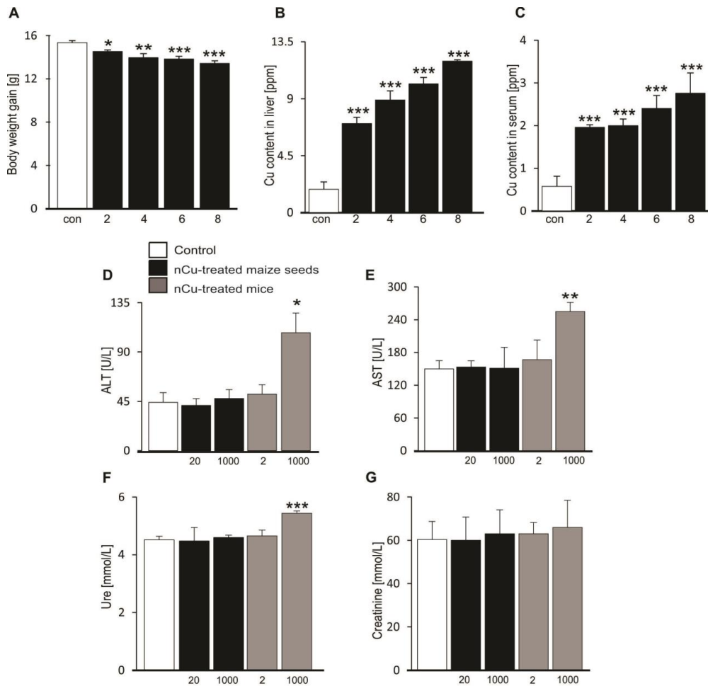
Figure 2. Effect of nano-copper on morphological and pathological changes in mice. A. Arithmetic means (n=4-5) of body weight gain in mice, which were left untreated (control, white bar) or treated with 1000 mg/l nCu (black bar) for indicated time intervals (2, 4, 6 and 8 weeks). * ( P<0.05 ), ** ( P<0.01 ) and *** ( P<0.001 ) represent significant differences from control group, ANOVA. B-C. Arithmetic means (n=4-5) of Cu content in liver (B) and serum (C) of mice, which were left untreated (control, white bar) or treated with 1000 mg/l nCu (black bar) for indicated time intervals (2, 4, 6 and 8 weeks). *** ( P<0.001 ) represents significant difference from control group, ANOVA. D-G. Arithmetic means (n=4-5) of serum alanine transaminase (ALT) (D), aspartate transaminase (AST) (E), urea (F) and creatinine (G) concentrations in mice, which were left untreated (control, white bars) or fed with grain maize derived from 20 mg/kg dry weight (DW) or 1000 mg/kg DW nCu-treated seeds (black bars) or treated with nCu at dose of 2 mg/l or 1000 mg/l (grey bars). * ( P<0.05 ), ** ( P<0.01 ) and *** ( P<0.001 ) represent significant differences from control group, ANOVA
