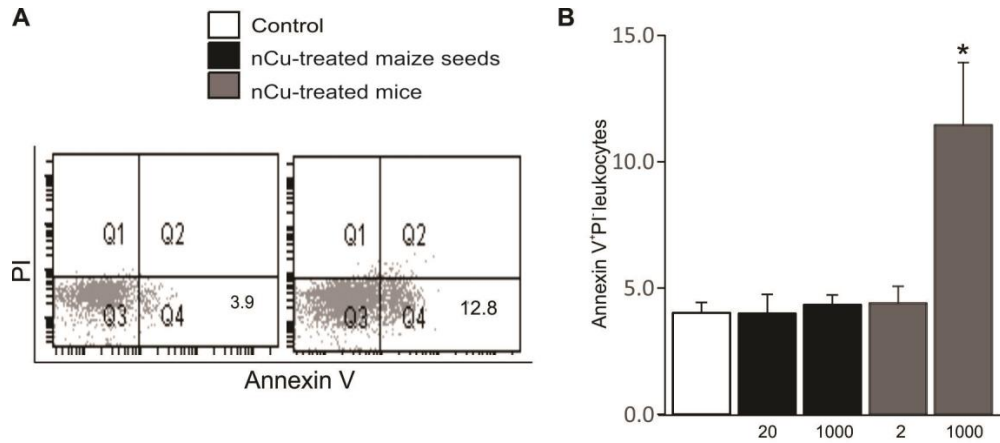
Figure 4. Effect of nano-copper on apoptotic death of splenic leukocytes in mice A. Original dot plots of Annexin V+ propidium iodide (PI)- leukocytes recruited to spleens of mice, which were untreated (control, left panel) and treated with 1000 mg/l nCu (right panel). Numbers depict the percent of cells in the respective quadrants, acquired within the dead cell gate B. Arithmetic means (n=5) of percentages of Annexin V+ PI- leukocytes recruited to spleens of mice, which were left untreated (control, white bars) or fed with grain maize derived from 20 mg/kg dry weight (DW) or 1000 mg/kg DW nCu-treated seeds (black bars) or treated with nCu at dose of 2 mg/l or 1000 mg/l (grey bars). * (P<0.05) represents significant difference from control group, ANOVA
