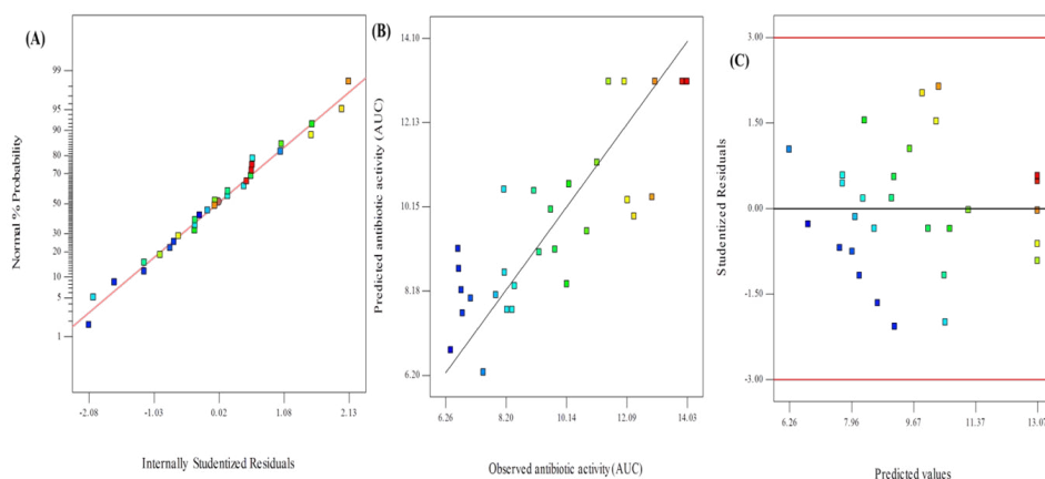
Figure 6. Diagnostic plots showing the model adequacy. (A) normal probability plot of the studentized residuals (B) Plot of observed response vs predicted response and. (C) Internally studentized residuals versus predicted response plot
