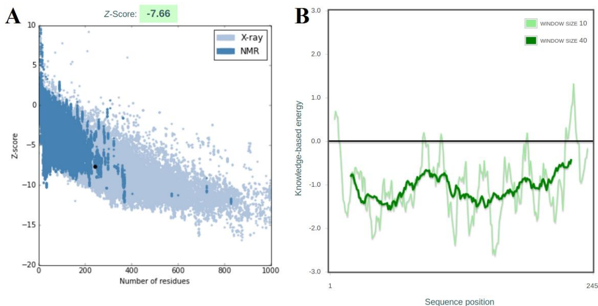
Figure 3. A) ProSA Z-score plot of modeled 3D structure of A9K. The bold black circle shows the position of this model among experimentally solved protein structures, which means that our predicted model is in the range of experimentally solved structures. B) Sequence position model quality. The more negative are indicative of the greater accuracy.
