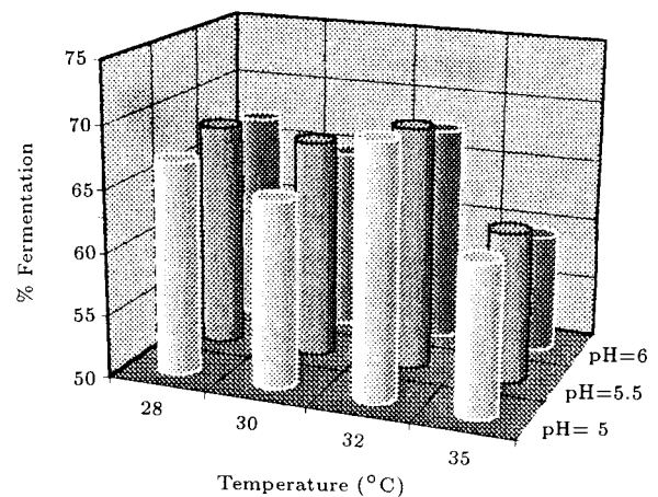
Figure 1c. Result of fermentation in batch reactor after 72 h.
