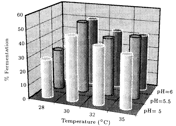
Figure 1a. Result of fermentation in batch reactor after 24 h.
