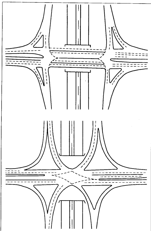
Figure 1. Geometric features of the SPUDI (top) and the CDI (bottom) [1].
