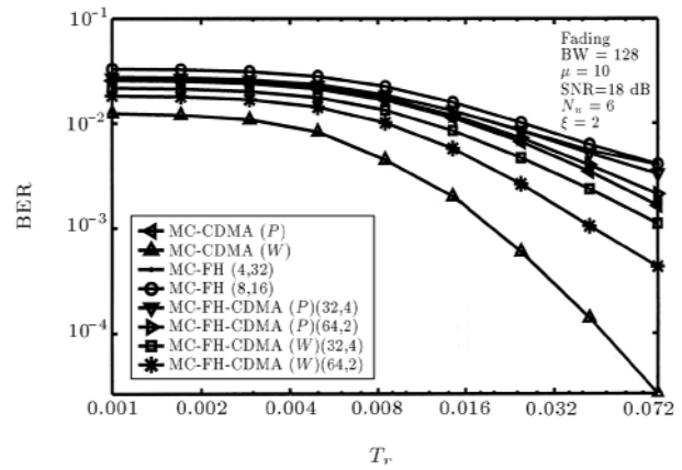
Figure 13. Performance of different systems in fading channels versus T_r with constant BW, \mu , SNR, N_u and \xi .
