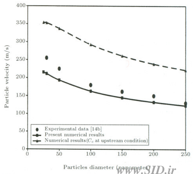
Figure 4. Comparison of the predicted particle velocities with the experimental data of Liu et al. [14] for different particle diameters.
