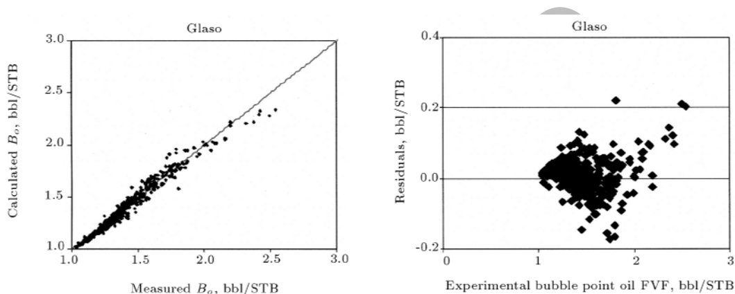
Figure 11. Cross plot and residual plot of B_o (Glaso [3]) based on Middle East PVT data.
