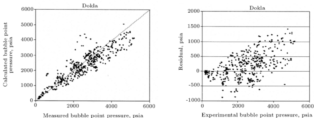
Figure 6. Cross plot and residual plot of P_b (Dokla [6]) based on Middle East PVT data.
