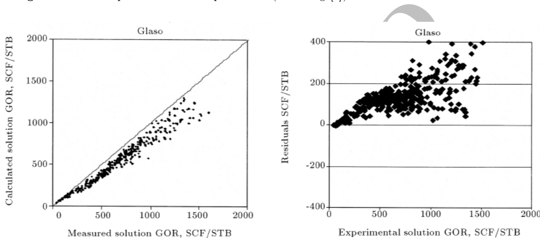
Figure 17. Cross plot and residual plot of R_s (Glaso [3]) based on Middle East PVT data.
