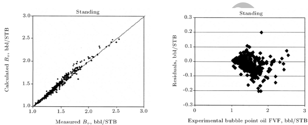
Figure 8. Cross plot and residual plot of B_o (Standing [1]) based on Middle East PVT data.
