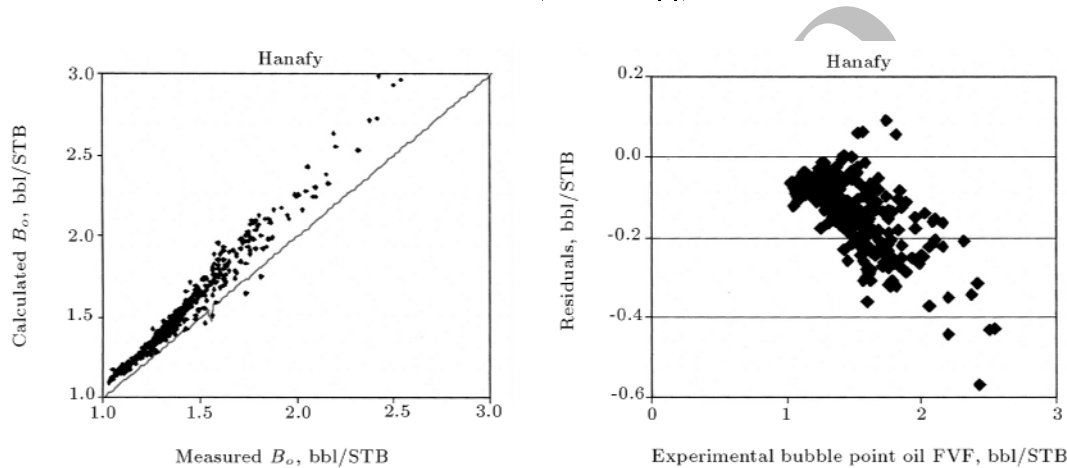
Figure 14. Cross plot and residual plot of B_o (Hanafy [7]) based on Middle East PVT data.
