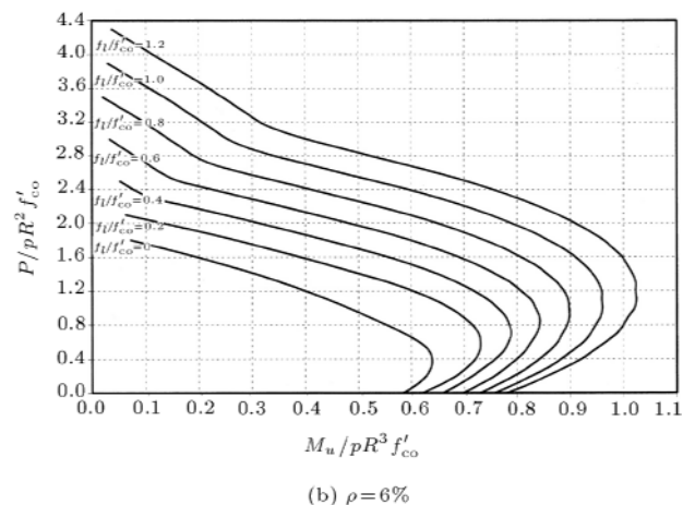
Figure 6. Typical moment capacity-axial force interaction curves.
