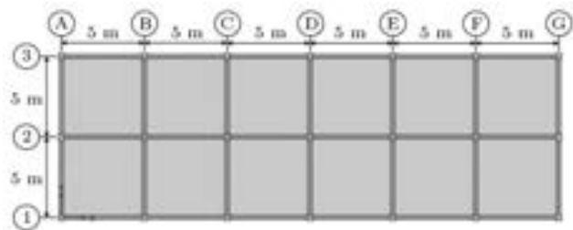
Figure 1. Plan of building without diaphragm opening (Model 4SEWNO).
