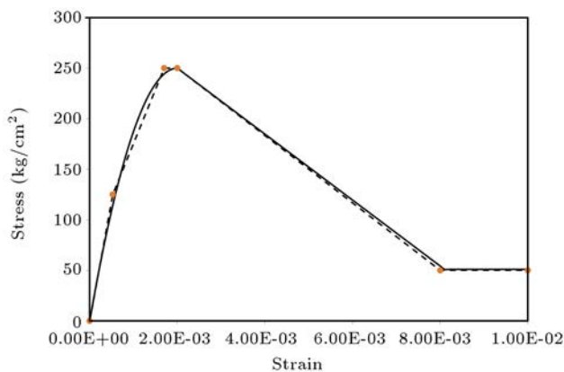
Figure 6. Concrete stress-strain relationship.
