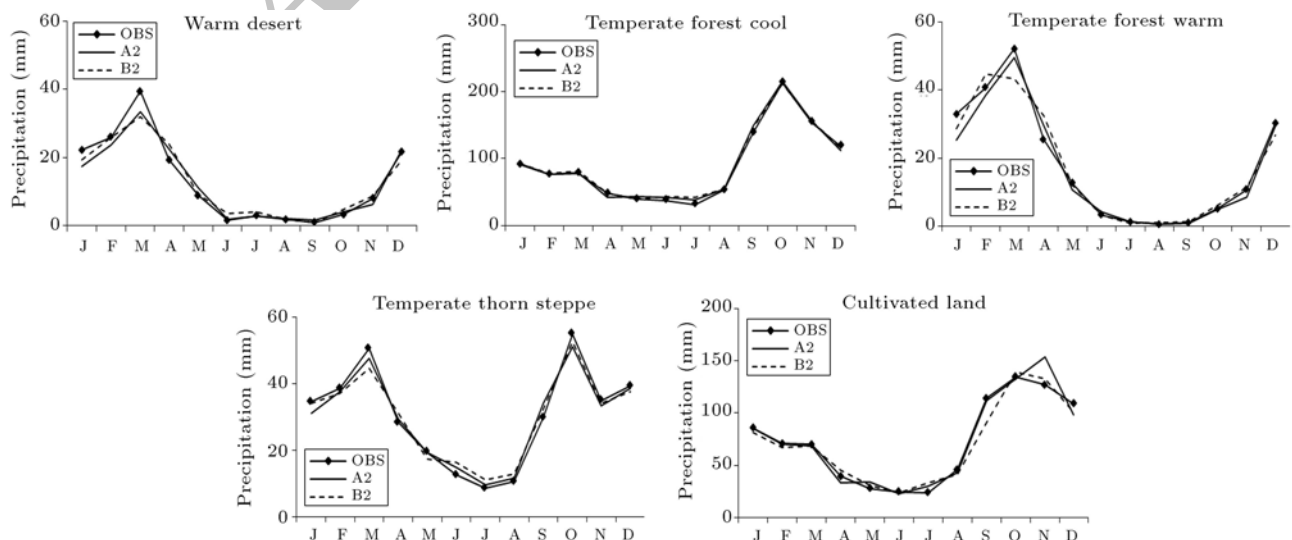
Figure 5. Comparison between observed data and A2 and B2 scenarios for monthly precipitation in different land uses.
