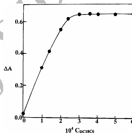
Figure 5. Effect of DC18C6 concentration in chloroform on the extraction of benzocaine. Conditions: benzocaine, 33 \mu\text{g/ml} ; H_2SO_4 , 2.5 \times 10^{-2} M; Calmagite, 2.0 \times 10^{-4} M.
