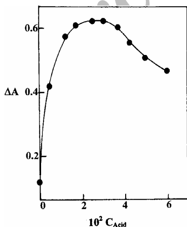
Figure 3. Effect of H_2SO_4 concentration on the extraction of benzocaine. Conditions: benzocaine 33 \mu\text{g/ml} ; calmagite, 2.0 \times 10^{-4} M; DC18C6, 2.010^{-4} M.
