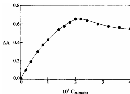
Figure 4. Effect of calmagite concentration on the extraction of benzocaine. Conditions: benzocaine 33 \mu\text{g/ml} ; H_2SO_4 , 2.5 \times 10^{-2} M; DC18C6, 2.0 \times 10^{-4} M.
