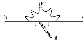
Figure 4. Feynman diagram for the gluonic penguin b \rightarrow sg^* . The gluon can be emitted from any of the quark lines and can be on-shell or off-shell.
