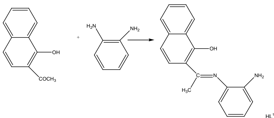
Scheme 1. Preparation of HL 1 .
