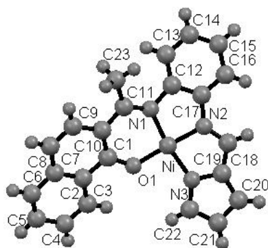
Figure 1. ORTEP drawing of NiL with the atom numbering scheme.
