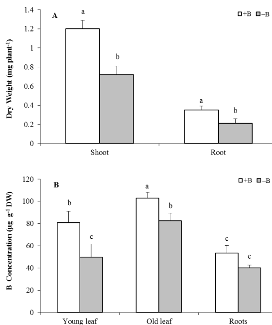
Figure 1. Dry weight ( mg\ plant^{-1} ) of shoot and root (A) and boron concentration ( \mu g\ g^{-1}\ DW ) (B) of three different fractions in B-sufficient (+B) and B-deficient (-B) tea ( Camellia sinensis L.) plants. Bars indicated by the same letter are not significantly different ( P < 0.05 ).
