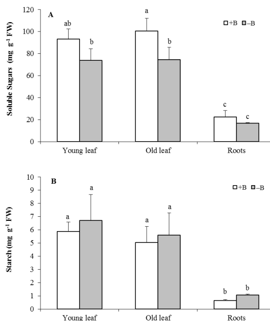
Figure 3. Concentration of soluble sugars (mg eq. glucose g -1 FW) (A) and starch (mg g -1 FW) (B) in the young and old leaves and roots of B-sufficient (+B) and B-deficient (-B) tea ( Camellia sinensis L.) plants. Bars indicated by the same letter are not significantly different ( P < 0.05 ).
