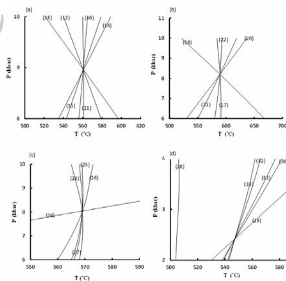
Figure 9. Stable intersections for M_1 assemblage containing phases of white mica, chlorite, biotite, plagioclase, staurolite, quartz and fluid. a) Stable intersection containing mu, cel, clin, daph, ann, fst, q and H_2O . b) Stable intersection containing mu, cel, clin, phl, ann, fst, q and H_2O . c) Stable intersection containing mu, clin, ames, phl, ann, east, fst, and H_2O d) Stable intersection containing mu, clin, ames, phl, ann, east, fst and H_2O .
