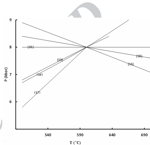
Figure 10. Cross cutting of independent reactions for M 1 assemblage.
