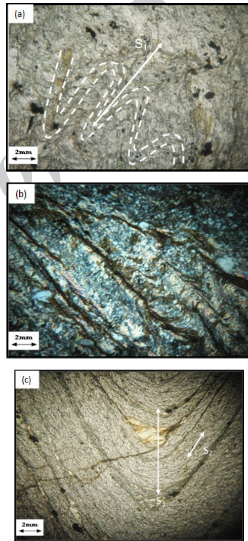
Figure 5. Photomicrograph of biotite-chlorite-muscovite schist showing a) S_1 schistosity b) S_2 schistosity c) S_2 and S_3 schistosity.
