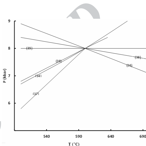
Figure 10. Cross cutting of independent reactions for M 1 assemblage.
