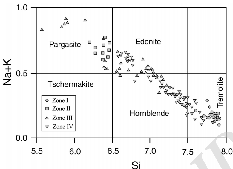
Figure 2. Classification of amphiboles in metabasites using Leake [20] diagram. All amphiboles from zone IV (orthopyroxene-clinopyroxene zone) plot in the hornblende and edenite fields.
