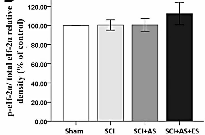
Fig.1. Western blotting analysis of phosphorylation of eukaryotic initiation factor 2 (eIf-2 \alpha ) and expression of Wingless-type3 (Wnt-3) proteins levels after 14 days in four experimental groups. (A) Experimental scheme. (B) Immunoblotting images of expression of Wnt-3 protein against \beta -actin and phospho-eIf-2 \alpha (p-eIf-2 \alpha ) against total eIf-2 \alpha . (C) Bar chart represents the quantified Wnt-3 protein bands in all experimental groups. The statistical one-way analysis of variance (ANOVA) of data showed the significantly elevated levels of Wnt-3 protein expression in the sub-threshold electrical stimulation (ES) group after 14 days. (D) Bar chart represents fold change of p-eIf-2 \alpha in all experimental groups. Analysis of results also, showed that the levels of eIf-2 \alpha phosphorylation in the sub-threshold ES group increased significantly after 14 days. * P=0.025 and *** P=0.00088 compared with the SCI+AS group (n= 10 rats per group).
