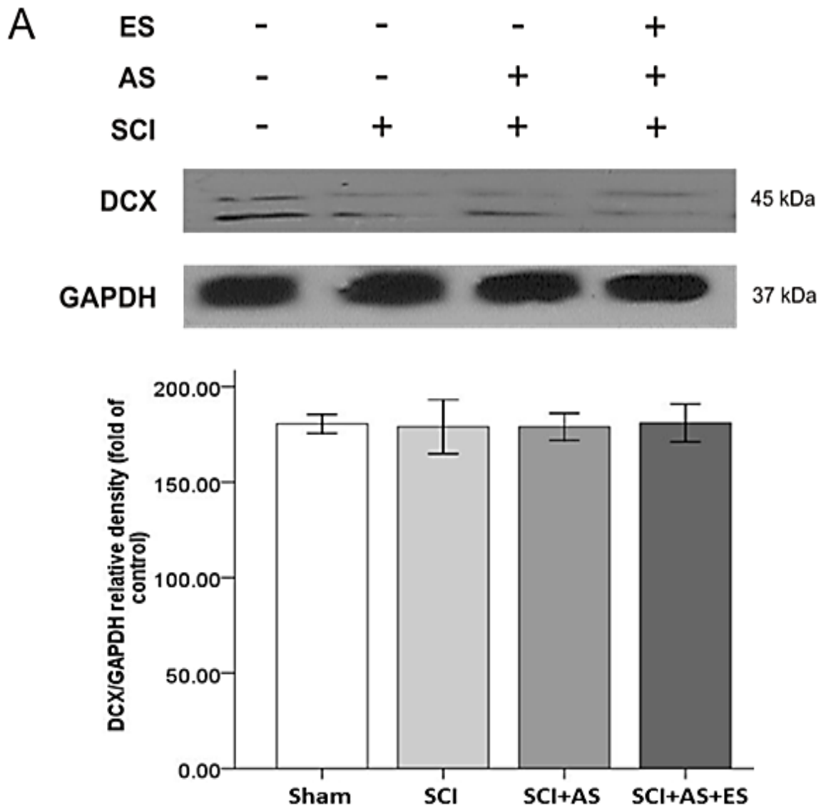
Fig.4. Effect of sub-threshold electrical stimulation (ES) on expression of doublecortin (DCX) protein in the spinal cord after 14 days in all experimental groups. (A) Immunoblotting images of DCX protein expression against glyceraldehyde 3-phosphate dehydrogenase (GAPDH) which considered as an internal standard. (B) Bars represent fold change of DCX protein (n= 10 rats per group).
