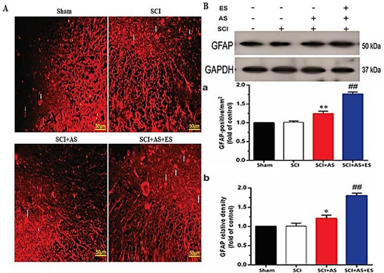
Fig.2. Glial fibrillary acidic protein (GFAP) expression after two weeks in four experimental groups in immunoblotting and immunohistochemical studies. (A) The fluorescent intensity of GFAP labeled cells after applying the sub-threshold electrical stimulation (ES) protocol in all experimental groups. Bar=50 microns. (B) Immunoblotting images of GFAP protein in the rat spinal cord for all experimental groups. (a) Quantified analysis of immunohistochemical images showed that in animals which received two weeks' period of ES, expression of GFAP marker significantly increased compared with spinal cord injury (SCI)+astrocyte (AS) cell group. (b) Bars illustrate fold change of GFAP protein normalized against glyceraldehyde 3-phosphate dehydrogenase (GAPDH) as an internal standard. As shown, the expression levels of GFAP protein in animals that received two weeks' period of sub-threshold ES was significantly enhanced versus SCI+AS group. * P=0.037 and ** P=0.011 compared with the SCI group. *** P=0.002 compared with the SCI+AS (n=10 rats per group). Magnification \times 40 .
