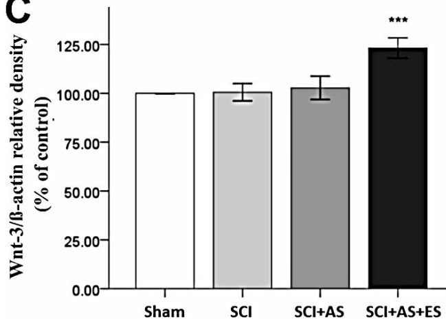
Fig.1. Western blotting analysis of phosphorylation of eukaryotic initiation factor 2 (eIf-2 \alpha ) and expression of Wingless-type3 (Wnt-3) proteins levels after 14 days in four experimental groups. (A) Experimental scheme. (B) Immunoblotting images of expression of Wnt-3 protein against \beta -actin and phospho-eIf-2 \alpha (p-eIf-2 \alpha ) against total eIf-2 \alpha . (C) Bar chart represents the quantified Wnt-3 protein bands in all experimental groups. The statistical one-way analysis of variance (ANOVA) of data showed the significantly elevated levels of Wnt-3 protein expression in the sub-threshold electrical stimulation (ES) group after 14 days. (D) Bar chart represents fold change of p-eIf-2 \alpha in all experimental groups. Analysis of results also, showed that the levels of eIf-2 \alpha phosphorylation in the sub-threshold ES group increased significantly after 14 days. * P=0.025 and *** P=0.00088 compared with the SCI+AS group (n= 10 rats per group).
