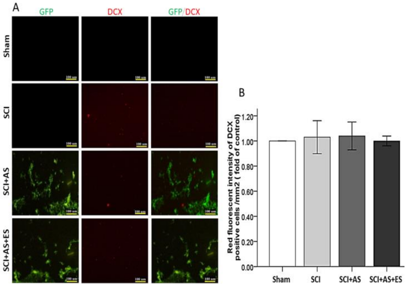
Fig.3. Immunohistochemical analysis of doublecortin (DCX) marker after two weeks in all experimental groups. (A) Doublecortin + (DCX + ) cells were not detected after 14 days in animal which received sub-threshold electrical stimulation (ES) as well as other groups Bar=100 microns. (B) Quantification analysis of DCX marker showed that there was no significant change in expression of DCX marker in all groups (n=10 rats per group). Magnification ×40.
