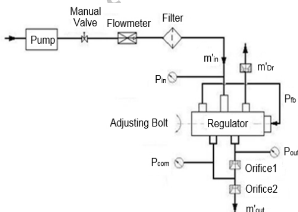
Figure 3. The hydraulic test circuit of regulator
