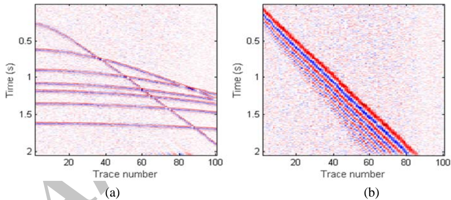
Figure 7. (a) The result of f-t-x filtering applied on shot gather, shown in Figure 4(b), to attenuate ground roll and suppress random noise. (b) The difference section or the eliminated noise.
