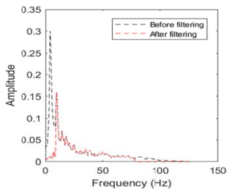
Figure 12. Average amplitude spectra related to synthetic shot gathers shown in Figures 11a (before filtering) and 11b (after filtering).
