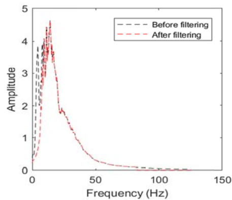
Figure 10. Average amplitude spectra related to synthetic shot gathers shown in Figures 9a (before filtering) and 9b (after filtering).
