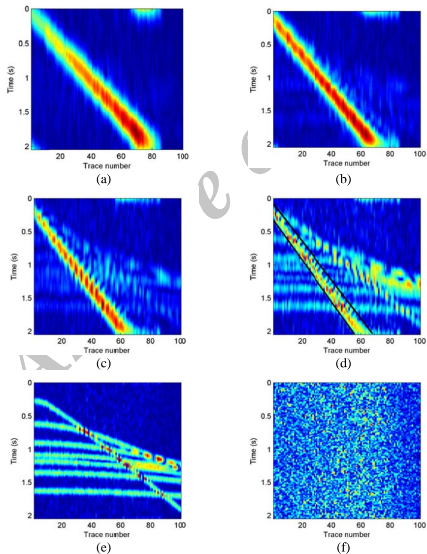
Figure 6. (a) to (f) show single-frequency t-x sections of frequencies 6 Hz, 9 Hz, 12 Hz, 15 Hz, 28 Hz and 80 Hz, respectively, analyzed from shot gather shown in Figure 4(c). As an example, the t-x distribution of ground roll is remarked on 15 Hz section (d) which needs to be filtered.
