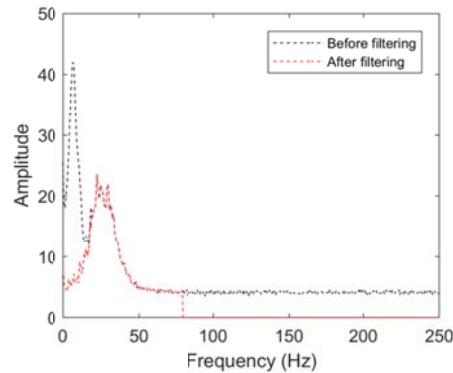
Figure 8. Average amplitude spectra related to synthetic shot gathers shown in Figures 4b (before filtering) and 7a (after filtering).
