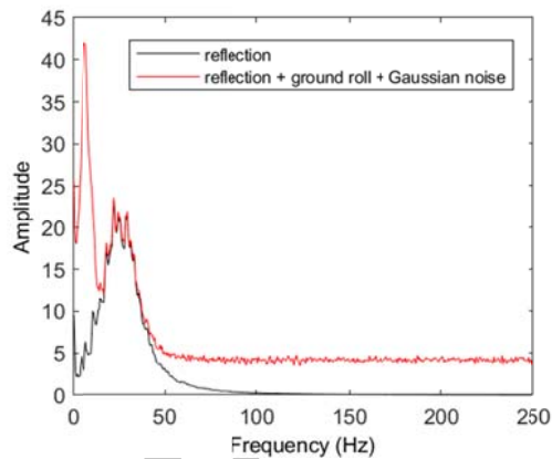
Figure 5. Average amplitude spectra related to synthetic shot gathers shown in Figures 4a (black) and 4c (red).
