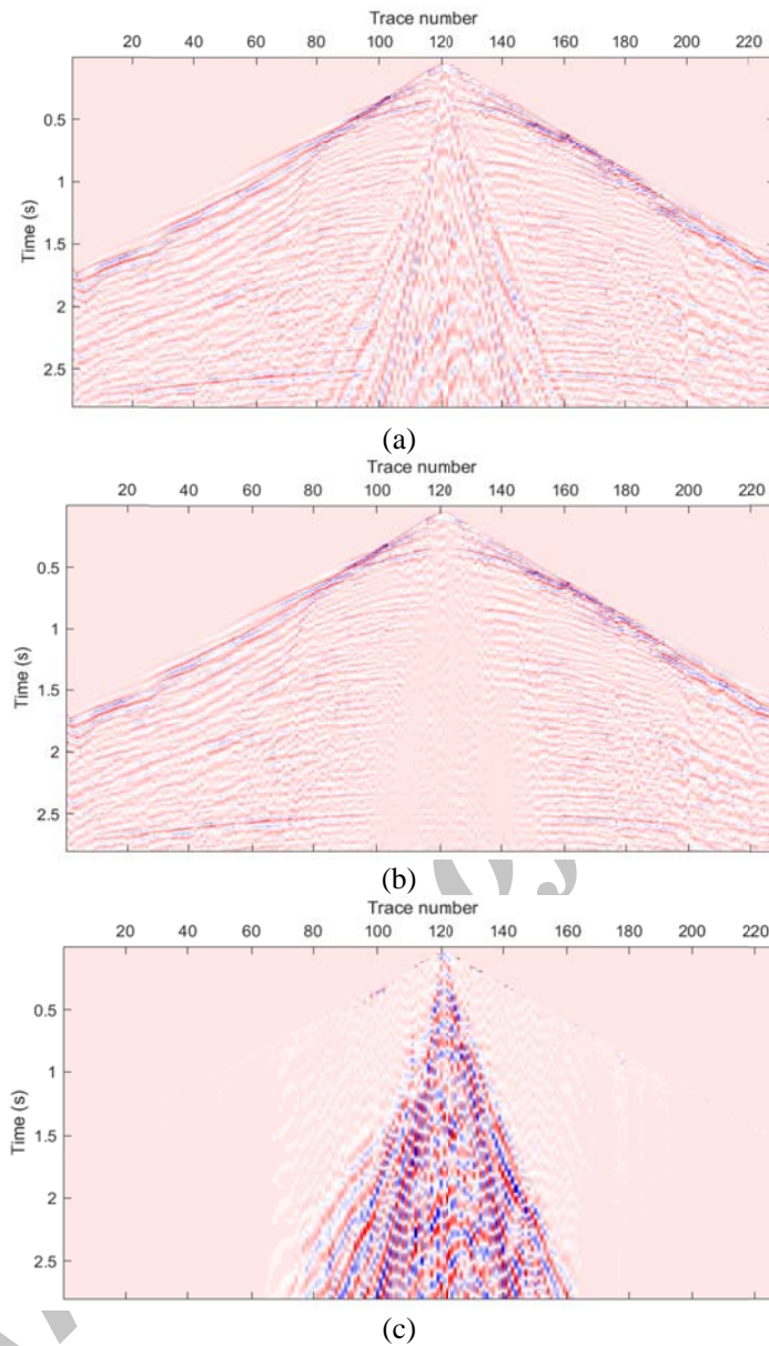
Figure 9. A real shot gather, before (a) and after (b) f-t-x filtering. The difference section of (a) and (b), as the removed noise is shown in (c).
