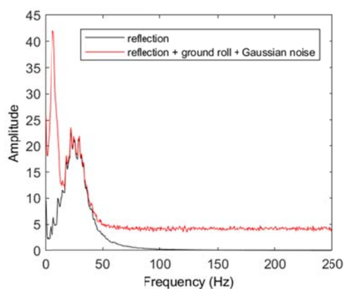
Figure 5. Average amplitude spectra related to synthetic shot gathers shown in Figures 4a (black) and 4c (red).
