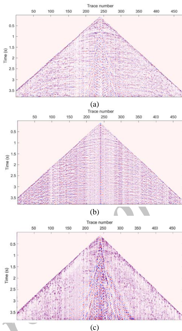
Figure 11. A real shot gather before (a) and after ground roll noise attenuation by proposed f-t-x filtering (b). The difference section of (a) and (b), as the removed noise (ground roll and random) is shown in (c). For better visualization of data, an AGC process to gain weak amplitudes has been applied to the figures.
