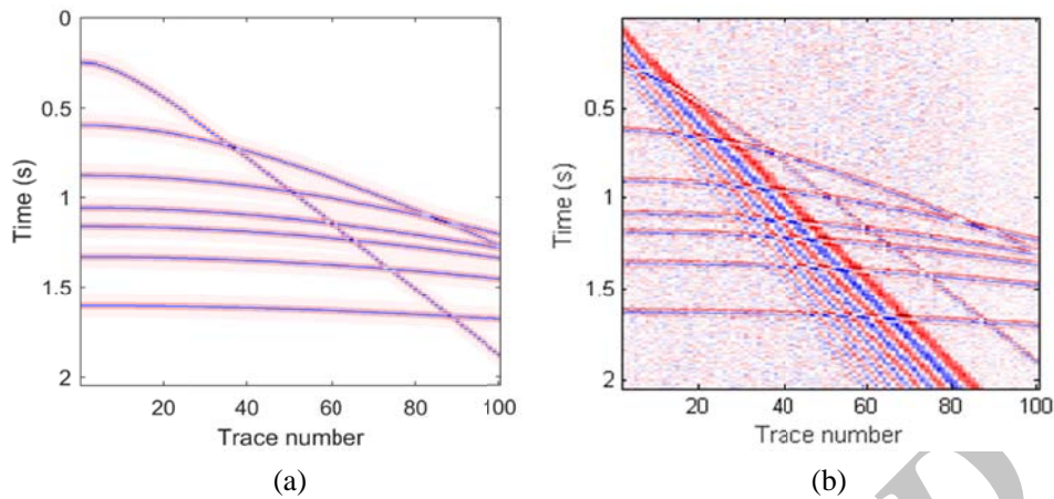
Figure 4. A synthetic seismic shot gather without any noise (a) and contaminated with ground roll and random noise (b).
