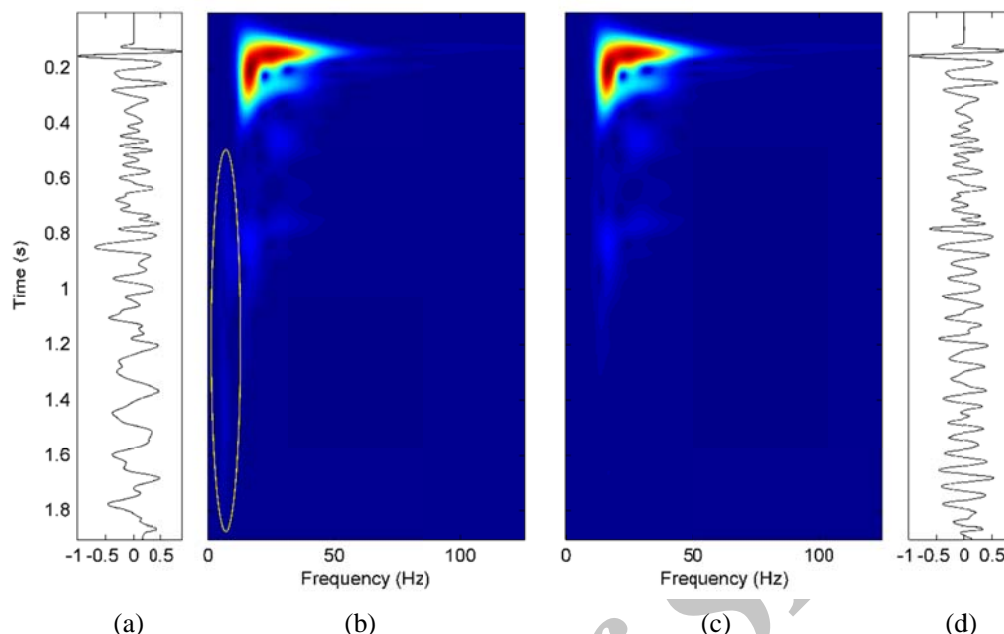
Figure 2. Ground roll attenuation in a sample seismic signal (a) by x-t-f filtering (Askari and Siahkoobi, 2008). (b) t-f map of (a) which in the ground roll distribution is remarked by yellow ellipse; (c) is filtered t-f map; and (d) filtered seismic signal constructing by inverse t-f transform of (c).
