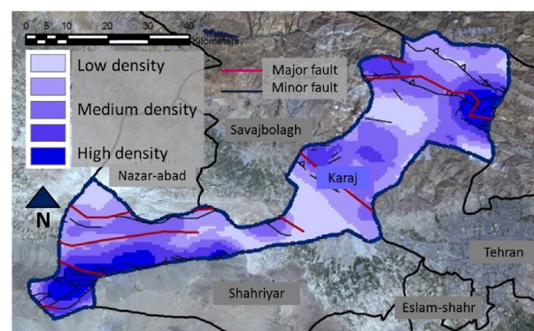
Figure 3. Fault map
