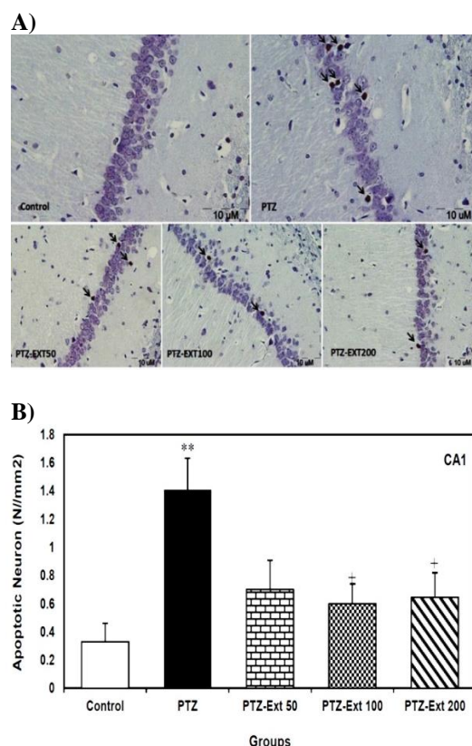
Figure 1. (A) Microscopic images of TUNEL-positive neurons (arrows) in the sections prepared from CA1 sub-region of hippocampus of different groups. TUNEL positive cells, as indicated by shrunk and brown nuclei, are scattered among normal neurons. (B) Comparison of the mean number of apoptotic neurons per unit area of CA1 sub-region in the control, PTZ-induced and pre-treatment groups (n=8). PTZ administration significantly increased the mean number of apoptotic neurons per unit area in comparison to the control group. However, only pre-treatment with 100 and 200 mg/kg of R. damascena extract led to significant decrease in the mean number of apoptotic neurons per unit area in comparison to PTZ-induced group. All data is presented as mean±SEM. **p<0.01 as compared to the control group; +p<0.05 as compared to the PTZ-induced group.
