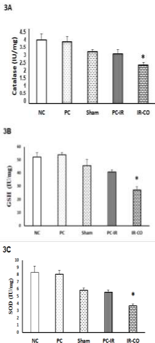
Figure 3. Effect of hepatic IR injury and p-coumaric pretreatment on catalase (3A), GSH (3B), and SOD (3C) in male Wistar rats. Hepatic IR injury decreased the levels of catalase, GSH, and SOD in liver tissue while pretreatment with p-coumaric acid increased these levels. * p < 0.05 versus sham, NC, PC and PC-IR groups. Data are presented as mean \pm S.E.M
