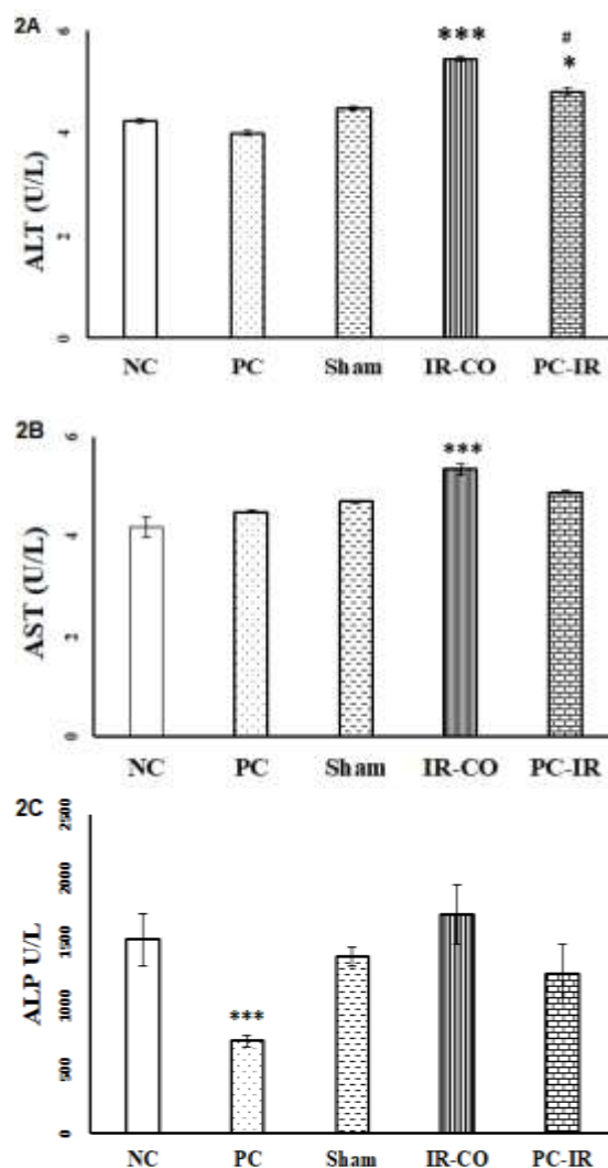
Figure 2. Effect of hepatic IR injury and p-coumaric pretreatment on ALT (2A), AST (2B), and ALP (2C) in male Wistar rats. Hepatic IR injury increased the levels of ALT, AST, and ALP while pretreatment with p-coumaric acid decreased these levels. NC (Normal intact group): these rats did not experience any surgical procedure. They received normal saline for seven days; Sham: Rats did not undergo hepatic IR injury. They received 7% DMSO (as vehicle) diluted in normal saline for seven days; PC and PC-IR groups: animals received p-coumaric acid (PC) at 100 mg/kg for the seven days; IR-CO and PC-IR: these groups underwent hepatic IR injury. *** p < 0.001 versus sham, NC and PC groups. # p < 0.01 compared to IR-CO rats and * p < 0.05 versus sham. Data are presented as mean±S.E.M.
