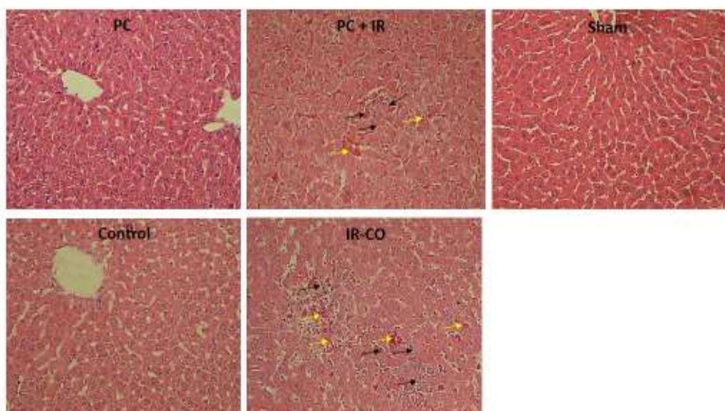
Figure 1. Microscopic representation of the liver tissue following IR injury (H&E staining \times 400 magnification). Yellow and black arrows respectively show hyperemia and inflammation.
