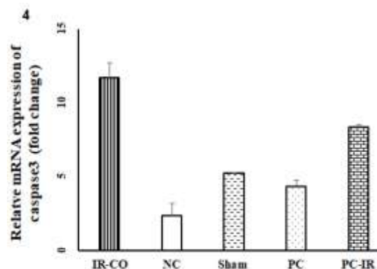
Figure 4. Effect of hepatic IR injury and p-coumaric acid pretreatment on caspase-3 mRNA expression level in male Wistar rats. Hepatic IR injury increased mRNA expression of caspase-3 in liver tissue while pretreatment with p-coumaric acid mitigated this increase. *** p < 0.001 versus NC, PC, and PC-IR groups. a p < 0.01 versus IR-CO group.
