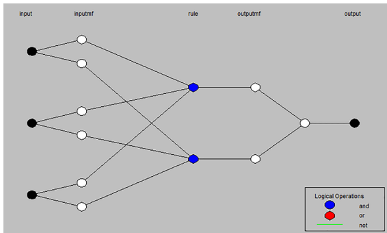
Figure 1: ANFIS arrays with two input membership functions
