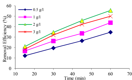
Fig. 6. Effect of nanoparticle concentration on COD removal
