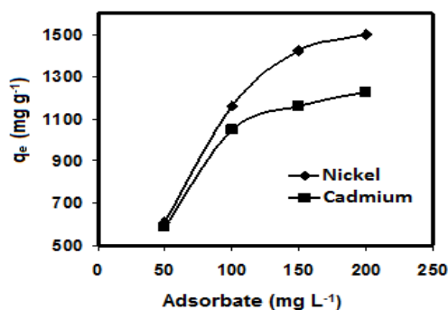
Fig. 6. Effect of initial heavy metal concentration on cadmium and nickel removal by PPI dendrimer (pH=7, C_{\text{adsorbent}}=0.08 g/L, T=298 °K)
