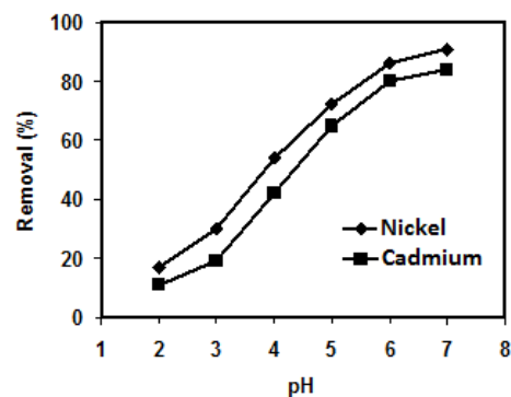
Fig. 4. Effect of pH on cadmium and nickel removal by PPI dendrimer ( C_0=100 mg/L, C_{adsorbent}=0.08 g/L, T=298 °K)
