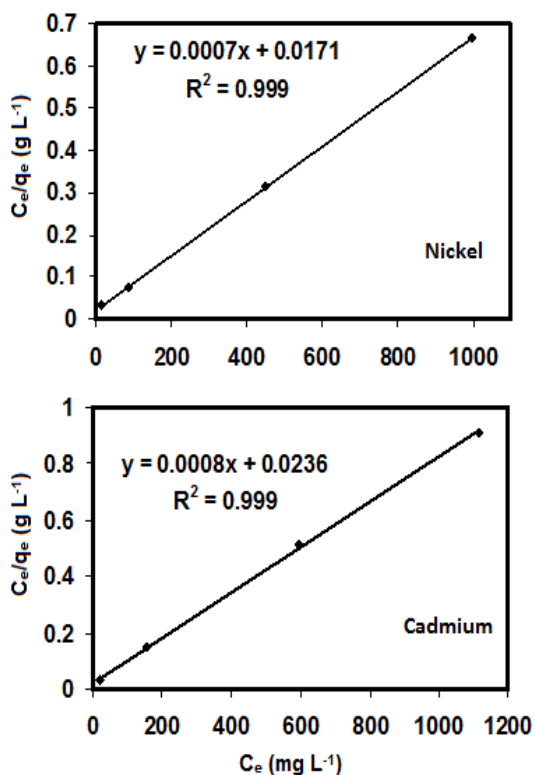
Fig. 7. Liner Langmuir isotherm of cadmium and nickel removal by PPI dendrimer (pH=7, adsorbent=0.08 g/L, T=298 °K)
