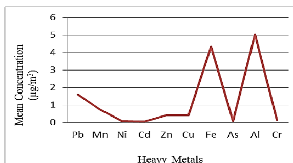
Fig. 4. Mean concentrations of heavy metals in indoor outdoor stations
