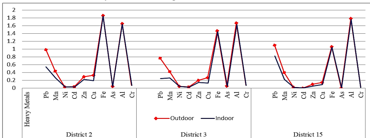
Fig. 6. Mean Concentration of Heavy Metals in Indoor and Outdoor Spaces of High-traffic Areas
