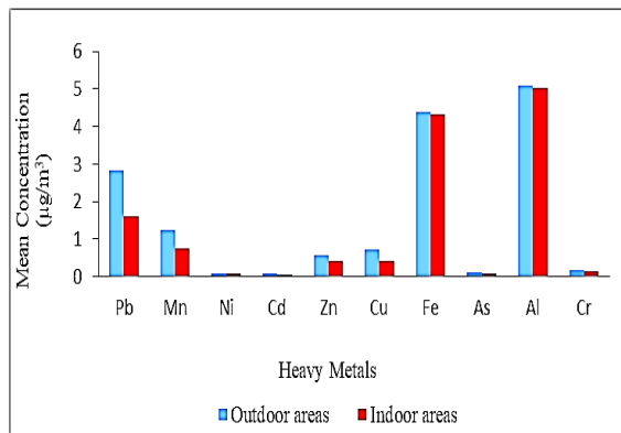
Fig. 5. Mean Concentration of Heavy Metals in Outdoor and Indoor Stations
