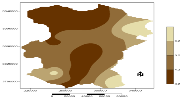
Fig.6. Zoning of soil quality of Gamasyab and Gharechay sub-basins
