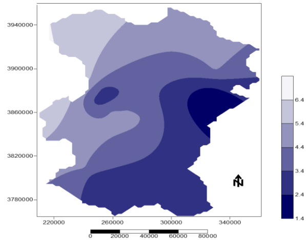
Fig. 5. Zoning of gravelius coefficients of Gamasyab and Gharechay sub-basins
