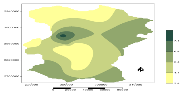
Fig. 7. Zoning of vegetation classification of Gamasyab and Gharechay sub-basins
