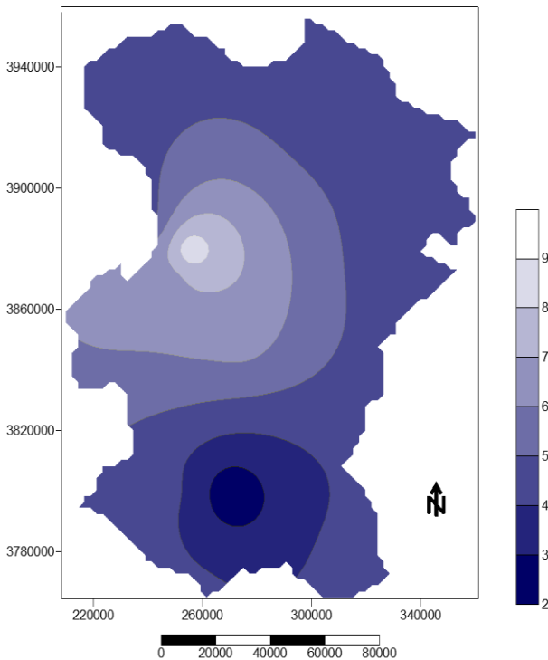
Fig. 3. Zoning of snow in Gamasyab and Gharechay sub-basins
