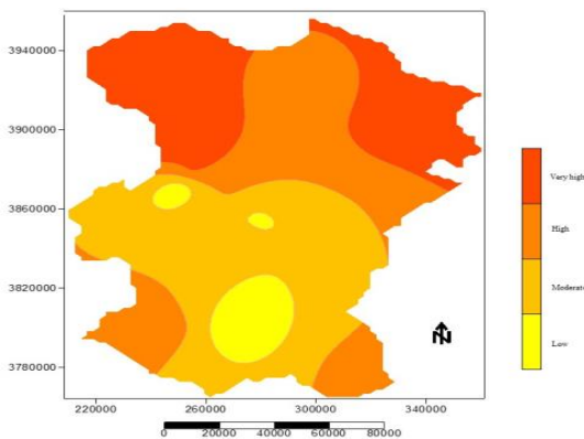
Fig. 8. Classification of flood intensity in Hamedan province
