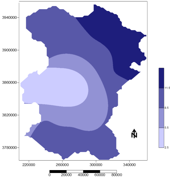
Fig. 2. Zoning mean maximum 24 h precipitation of Gamasyab and Gharechay sub-basins
