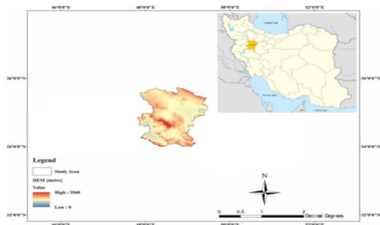
Fig. 1. The geographical location of Hamadan Province
