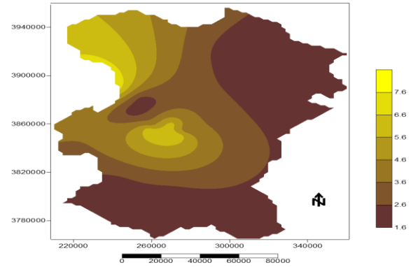
Fig. 4. Zoning of sub-basin slope in Gamasyab and Gharechay sub-basins
