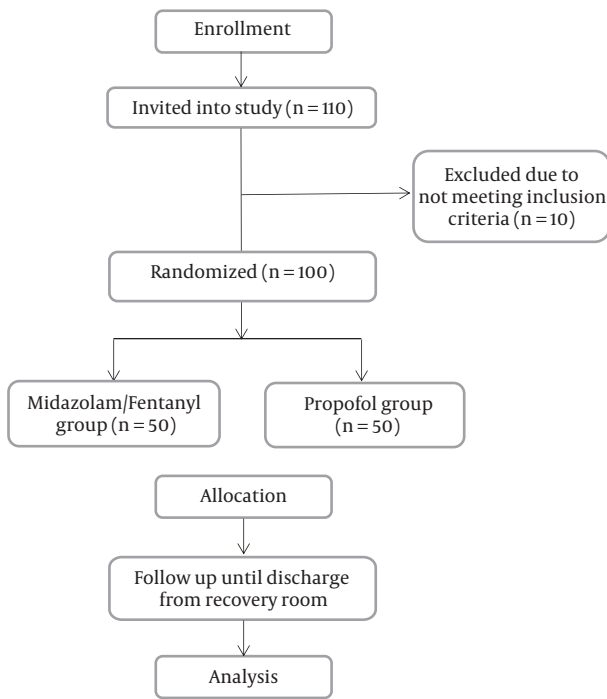
Figure 1. RCT flowchart
