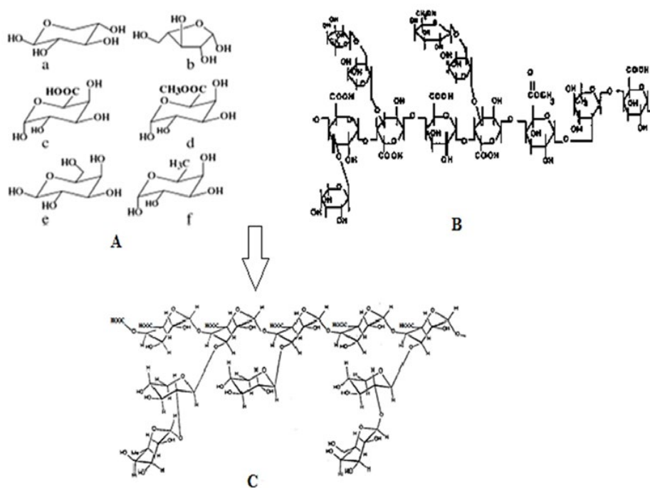
Fig. 1: (A) Main chemical building units of the GT \beta -D-xylose L-arabinose, \alpha -D-galacturonic acid, d) \alpha -D-1-galacturonic acid methyl ester) \beta -Dgalactose )1 \alpha -L-1-fucose, (B) The main structural of GT, (C) Structure of Bassorin [4]
