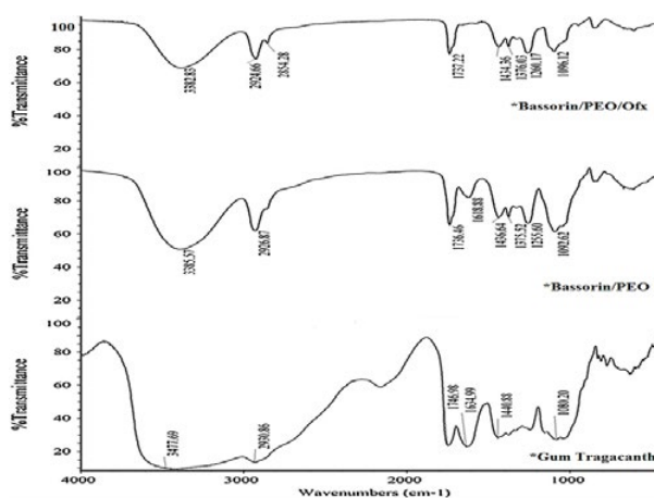
Fig. 4: FTIR spectra of Gum Tragacanth, Bassorin/PEO nanofibers and Bassorin/PEO/Ofx nanofibers
