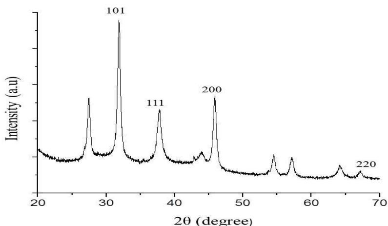
Fig. 2. The image represents the crystalline silver nanoparticles
