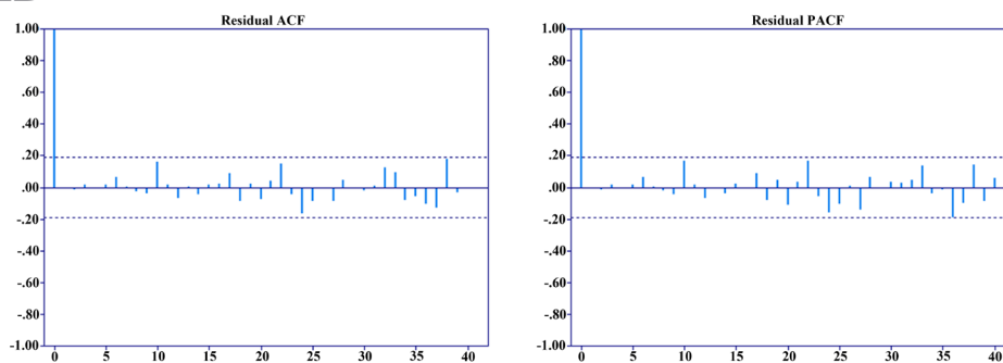
Figure 2. Residual graph of ACF and PACF for assessing fitness of selected model.
