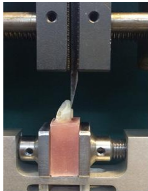
Figure 1. Sample being tested in a universal testing machine
