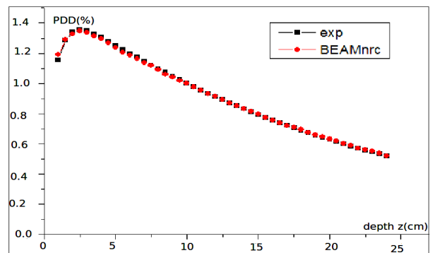
Figure 2. BEAMnrc and experimental PDD curve in the water phantom for 10x10 cm 2 field size for 12 MV beam.
