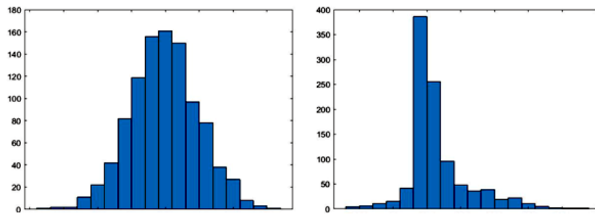
Figure 2. The Asymmetry Number is a Sign of Irregularity in the RR Interval Signal.
