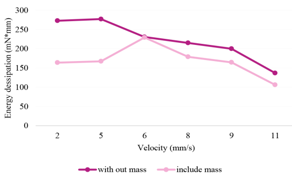
Figure 6. Energy Dissipation of Normal and Cancerous Tissues in Simple Stimulation at Different Velocities and Probe Location. Vertical and horizontal axes show energy dissipation and velocity (mm/s), respectively..
