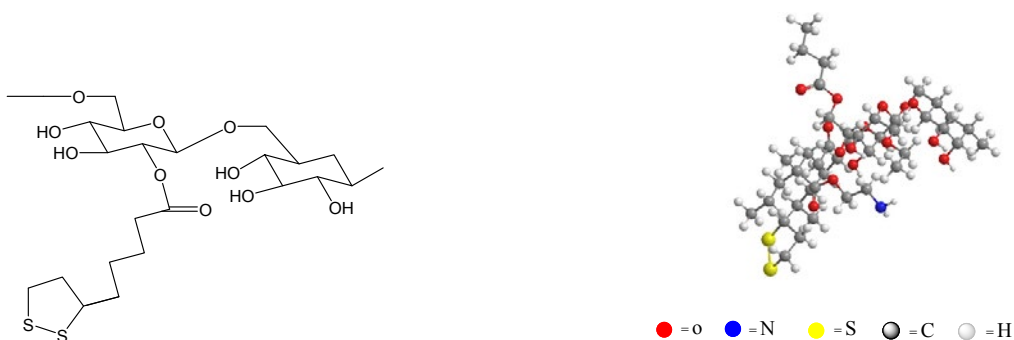
Fig. 2. Pre-polymer structure of lipico acid-dextran
