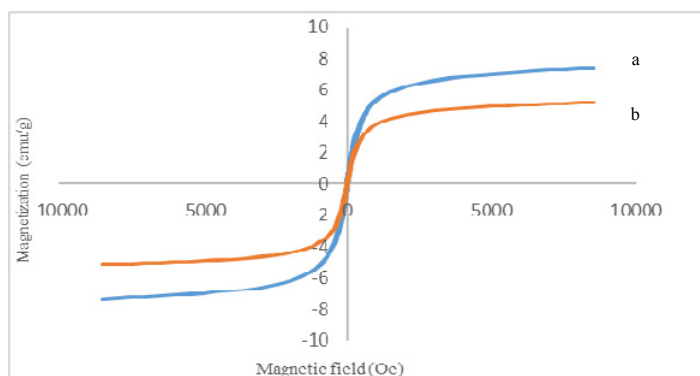
Fig. 2. Magnetization hysteresis loop behavior of Fe_3O_4 (a), Fe_3O_4@[NVC][AP] (b)
