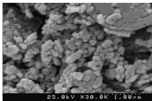
Fig.1. Nano-ZnO image provided by the SEM.
